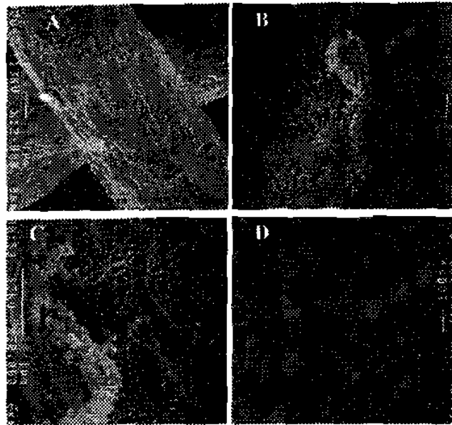
Fig. 4. Scanning electron micrographs of P. aphanidermatum induced by P. fluorescens Q2-87 producing 2,4-DAPG, during the time-course of hyphal degradation, in the intermediate area where diffusible bacterial antibiotic and Pythium are interacting. Mycelial hypha was grown in single culture for 24 h showing normal hypha with a much rougher outer surface (A) compared to that grown in a dual culture (B). Mycelial hypha was grown in single culture (C) for 48 h compared to that grown dual culture (D) showing a relatively smooth cell wall relative to that in control. Mycelial hypha was grown single culture (E) for 72 h compared to that grown in dual culture (F) which show a smooth outer layer of the cell wall. Mycelial hypha was grown in single culture (G) for 96 h compared to that grown in dual culture (H) which show looseness and disconnection of the outer layer of the cell wall. Magnifications were indicated within the Figs.
