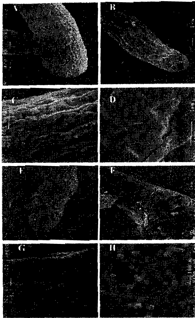
Fig. 2. Scanning electron micrographs of P. ultimum induced by P. fluorescens Q2-87 during the time-course indicated of cell wall hyphal degradation, in the intermediate area where diffusible bacterial antibiotic and Pythium are interacting. Mycelial hypha was grown in single culture for 24 h having normal growth and much rougher outer surface (A) compared to that grown in dual culture showing less rougher outer surface (B). Mycelial hypha was grown in single culture (C) for 48 h compared to that grown in dual culture (D) showing relatively smooth cell wall relative to the control. Mycelial hypha was grown in single culture (E) for 72 h compared to that grown in dual culture (F) showing looseness and disconnection of the outer layer of the cell wall. Mycelial hypha was grown in single culture (G) for 96 h compared to that grown in dual culture (H) showing complete degradation of the outer layer, at least, of the cell wall and revealing wall microfibril skeleton. Magnifications were indicated within Figs.
