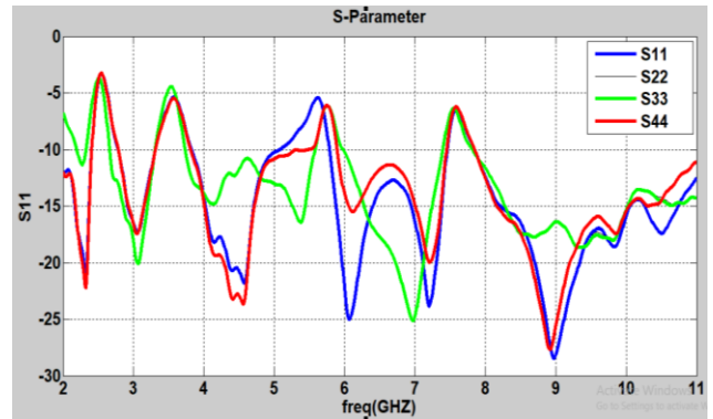
Fig. 4: The S_{11} , S_{22} , S_{33} and S_{44} of the MIMO antenna design with four-notched bands
