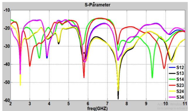
Fig. 5. S-parameter of MIMO antenna S_{12} , S_{13} , S_{14} , S_{23} , S_{24} and S_{34}
