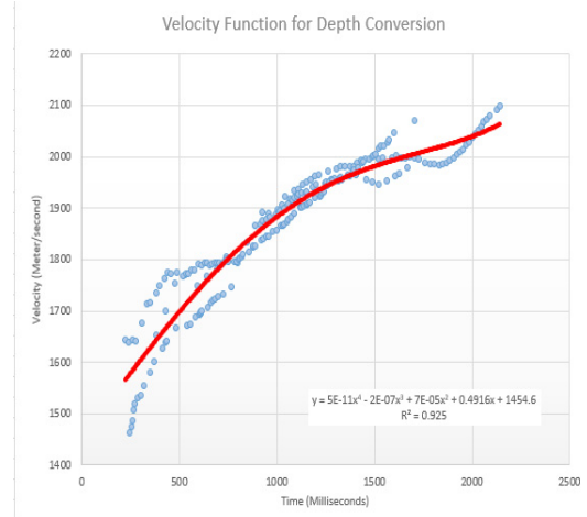
Fig. 14. Velocity function used for depth conversion using the integrated time depth tables after sonic calibration.
