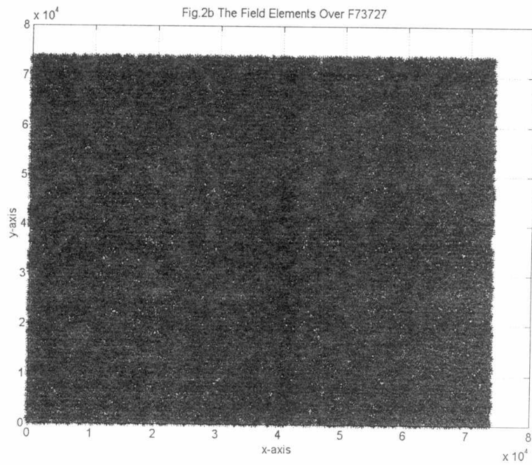
Fig.2 illustrates an example of the field elements over F2579, and F73727 respectively.
