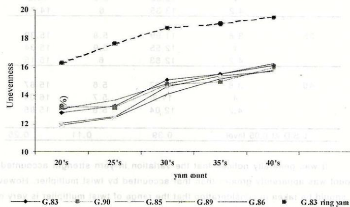
Fig 3. Effect of yarn count on yarn unevenness of Open-End spun yarn (4 cottons) and ring-spun Giza 83
