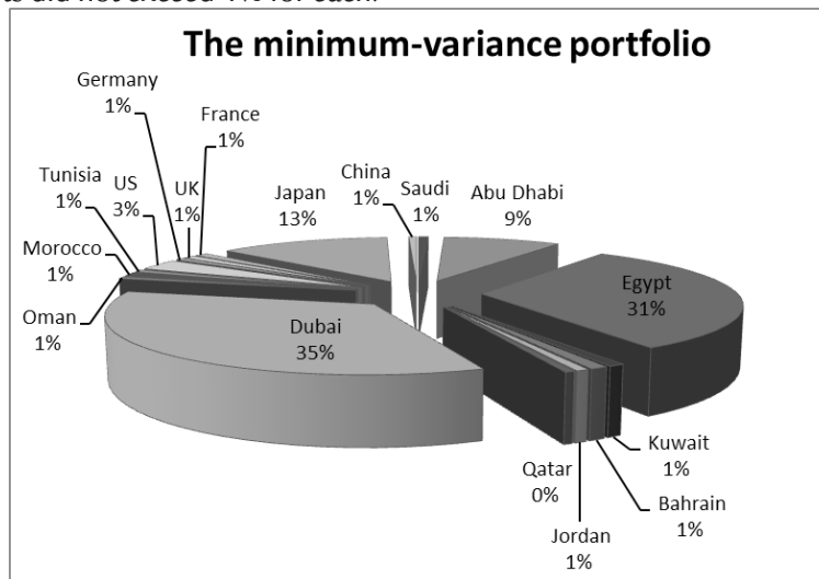
Figure (7) Weights of the Minimum-variance International Portfolio
