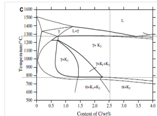
Fig. 1.c: Fe-C-Cr system with 20 % Cr.
