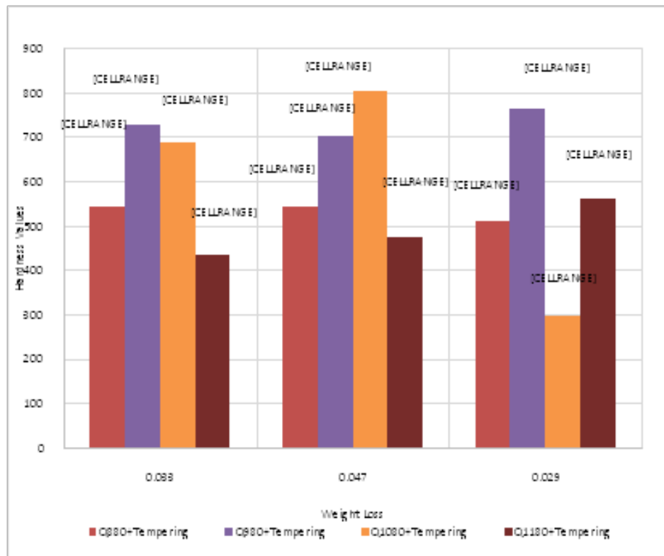
Fig. 9: Effect of the destabilization temperature following by tempering on the mechanical properties for high chromium white cast iron
