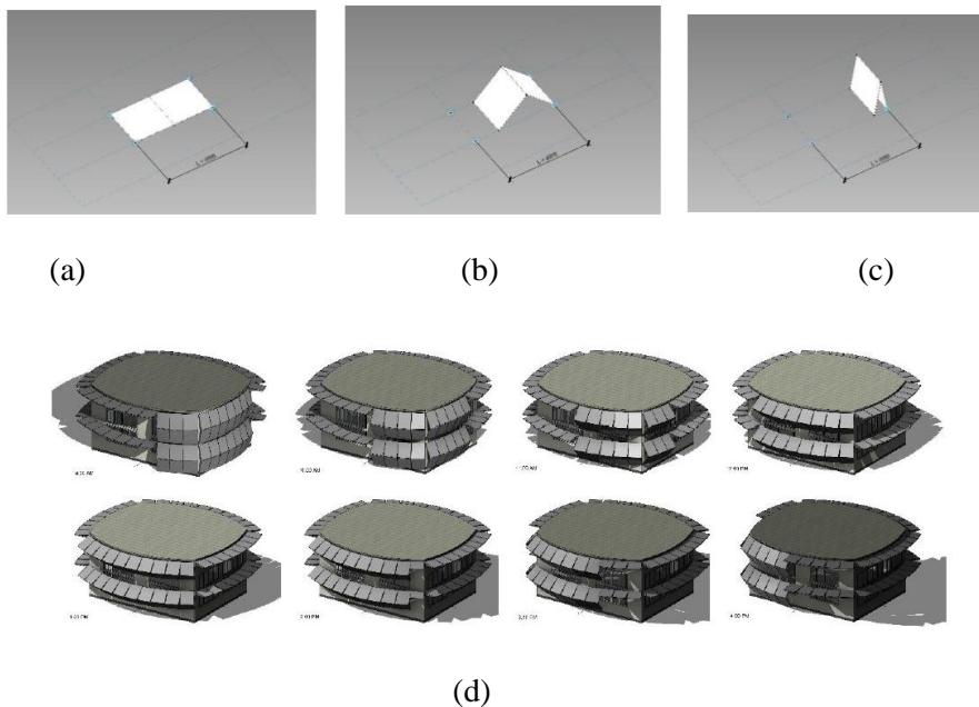
Fig. 5 (a) Angle = 0, (b) Angle = 45, (c) Angle = 85, (d) units positions as example from 9 AM to 4 PM, December 21
