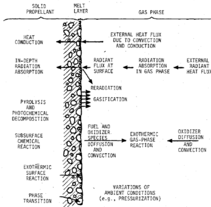
Figure 1. Physical processes involved in solid propellant ignition [4].
