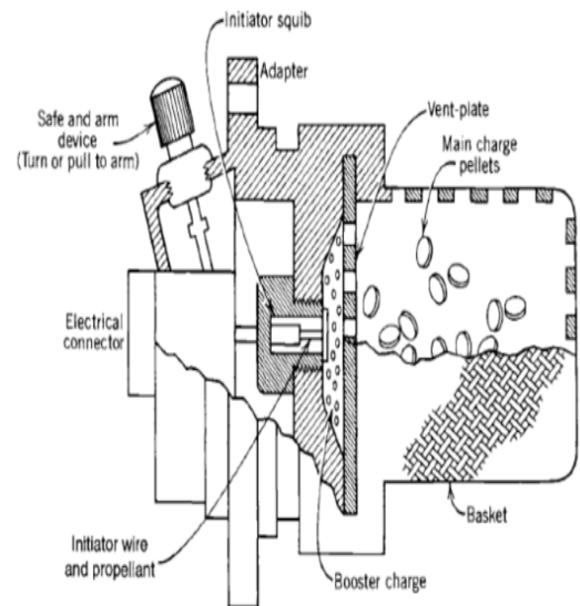
Figure 3. Pyrotechnic igniter [3].
