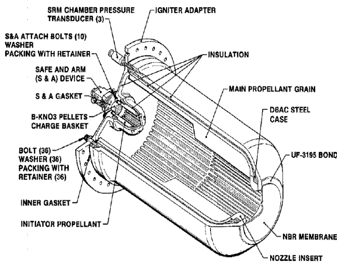
Figure 8. SRM Igniter
