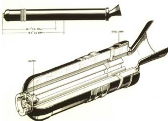
Figure 11. Motor No.7 [14].
