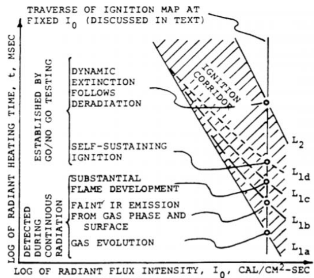
Figure 7. Ignition corridor [9].
