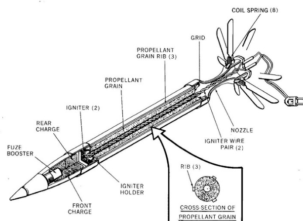
Figure 12. Motor No. 1 [15].
