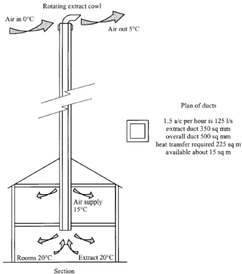
Figure 3 Small house natural ventilation with heat reclaims (A very tall chimney)
