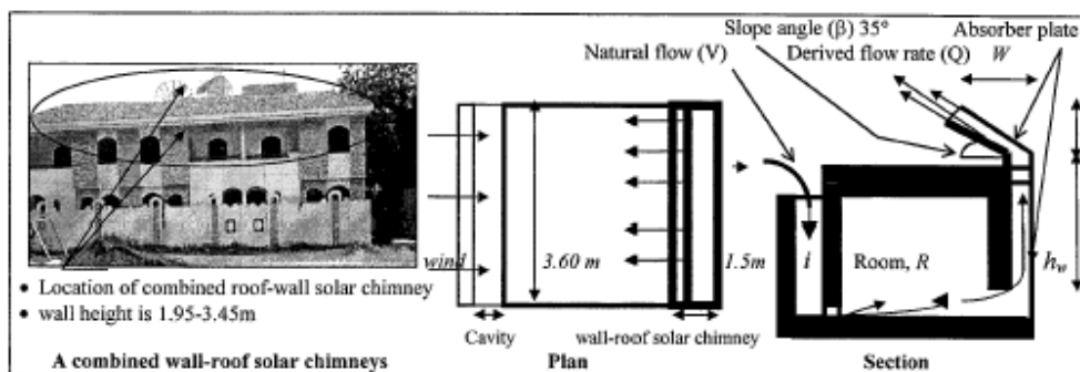
Figure 7 A combined wall-roof solar chimney incorporated into a residential building
