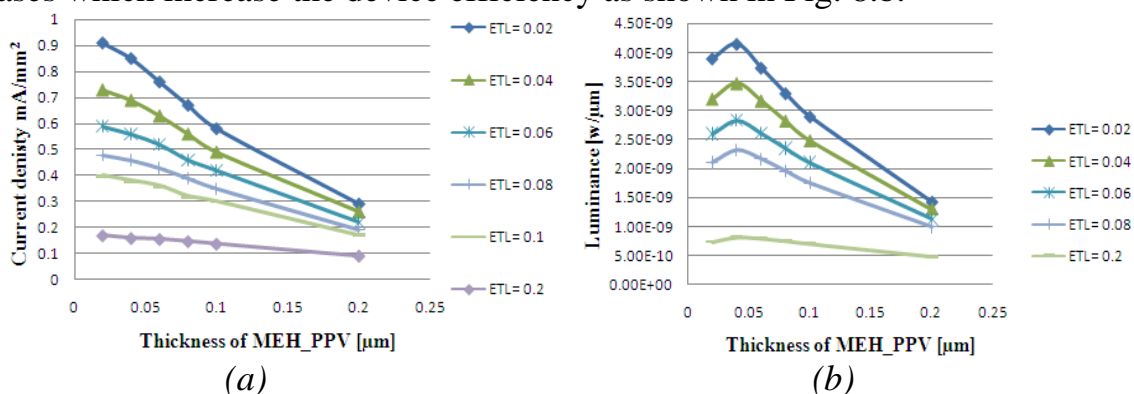
Fig. 8: (a) Current densities (b) Power of luminance for ITO/MEH-PPV/ETL/LiF-Al with different thicknesses of MEH-PPV and ETL
