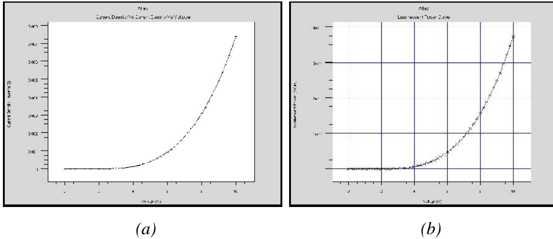
Fig. 9: Simulation results of ITO/Alq3 100nm/NPB 100nm/Lif-AL, (a) J-V curve, (b) power of luminance
