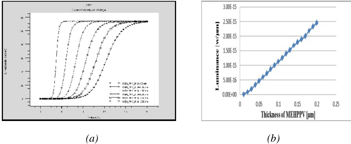
Fig. 4: (a) current densities, (b) Luminance for ITO/MEH-PPV//LiF-Al with different thicknesses of MEH-PPV
