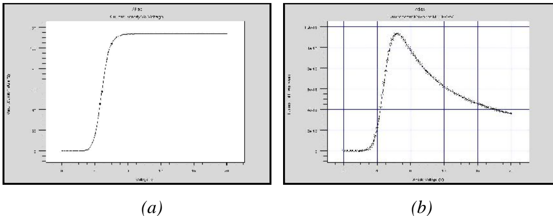
Fig. 3: simulation results of ITO/MEH-PPV 100nm /LiF-AL, (a) J-V curve, (b) power of luminance
