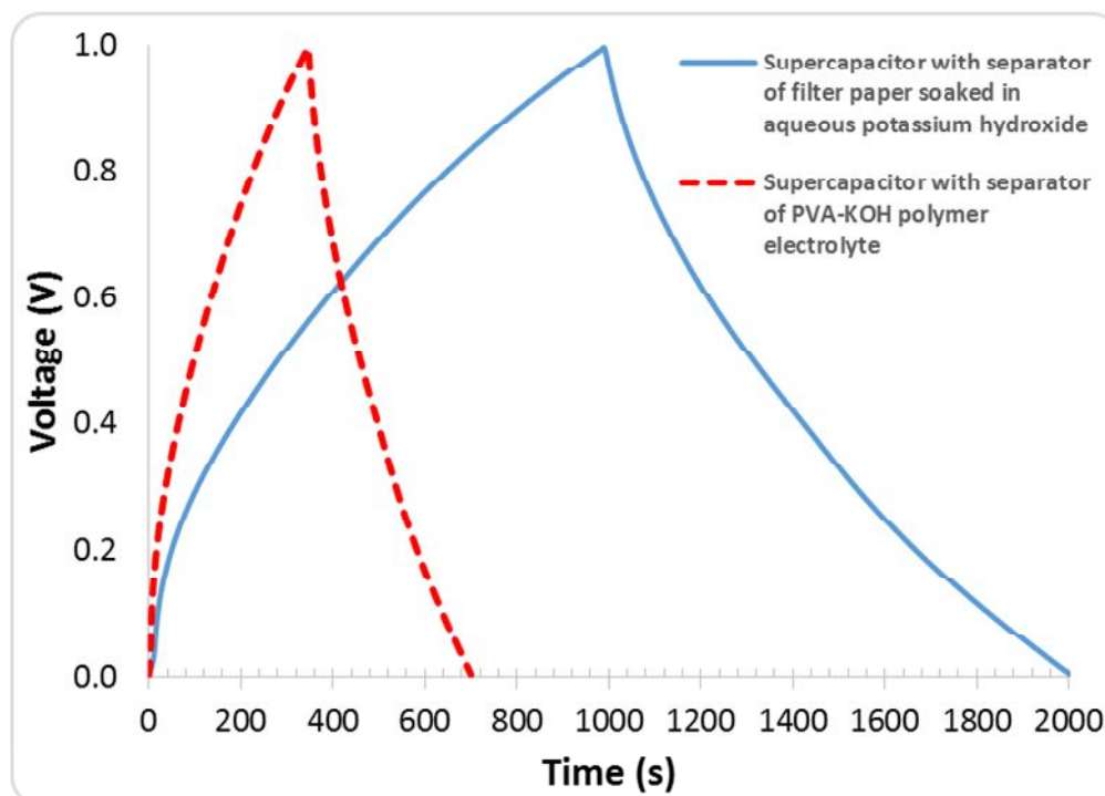
Figure (6): Charge-discharge curves at constant current of 3.5 mA of asymmetric supercapacitor with separator of filter paper soaked in aqueous potassium hydroxide and PVA-KOH polymer electrolyte
