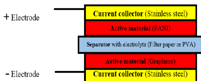
Figure (1): Fabricated supercapacitor structure
