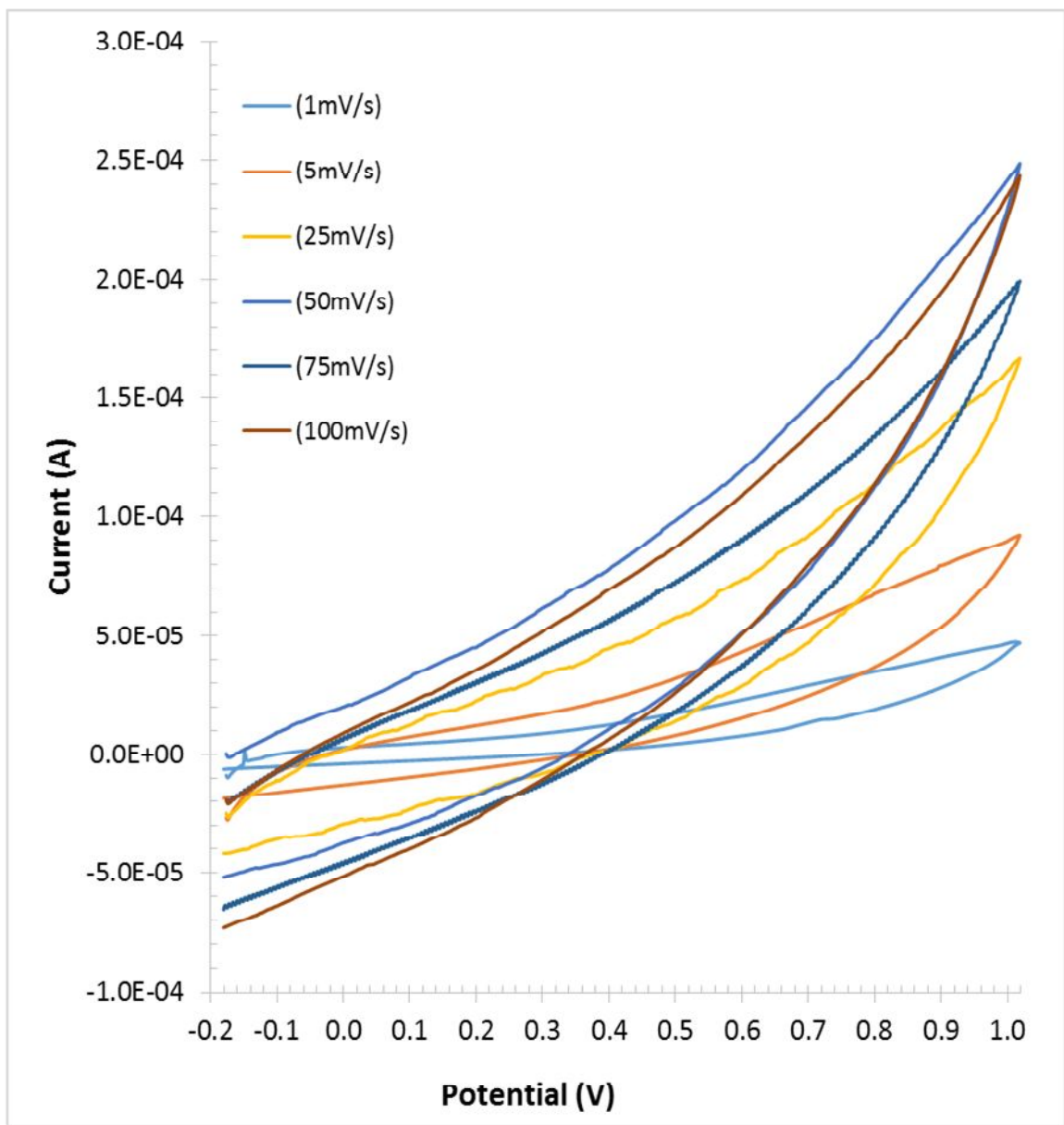
Figure (3): CV asymmetric supercapacitor with separator of PVA-KOH polymer electrolyte
