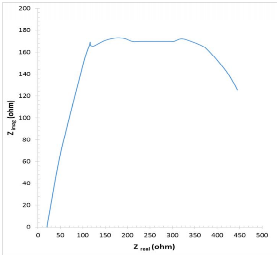
Figure (5): Nyquist plot of asymmetric supercapacitor with separator of PVA-KOH polymer electrolyte
