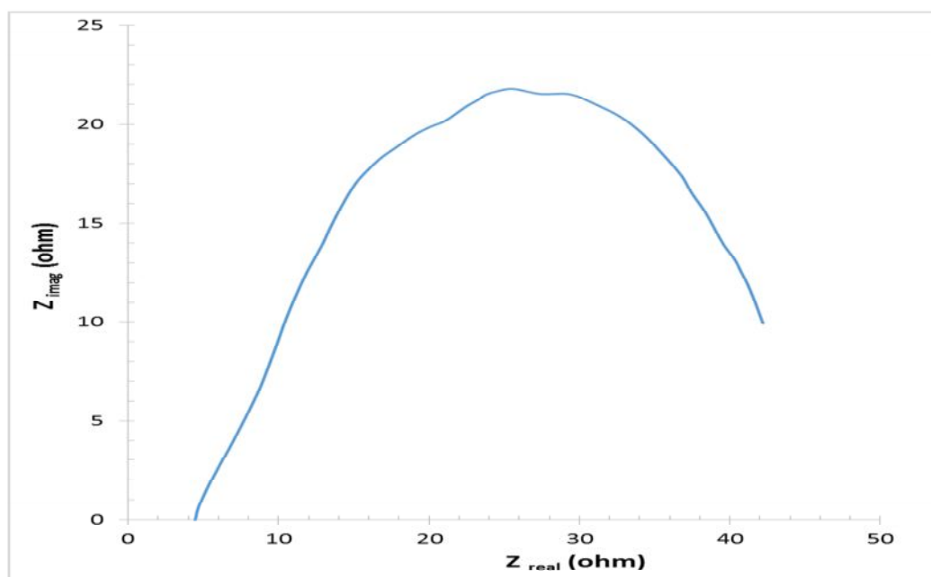
Figure (4): Nyquist plot of asymmetric supercapacitor with separator of filter paper soaked in aqueous potassium hydroxide
