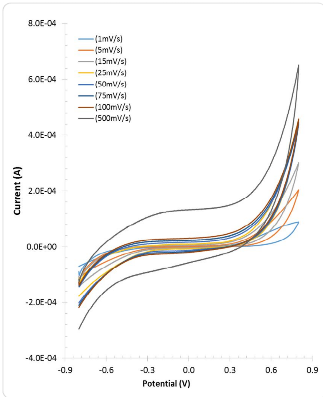
Figure (2): CV of asymmetric supercapacitor with separator of filter paper soaked in aqueous potassium hydroxide
