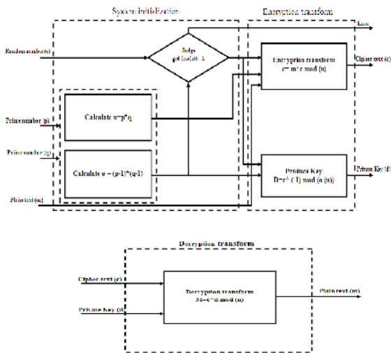
Figure 1. Block diagram of RSA encryption and decryption algorithms
