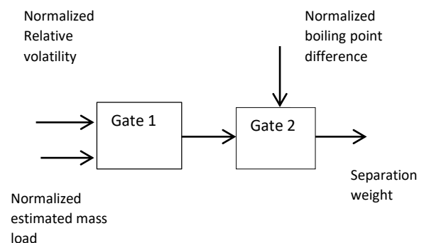
Figure 1 fuzzy analogical gate network
