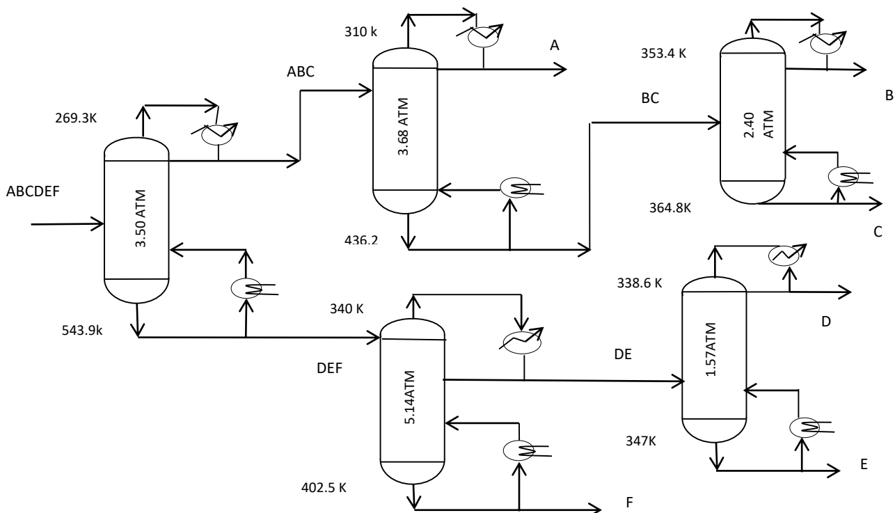
Figure 4 Flow sheet of the separation sequence for case study 1
