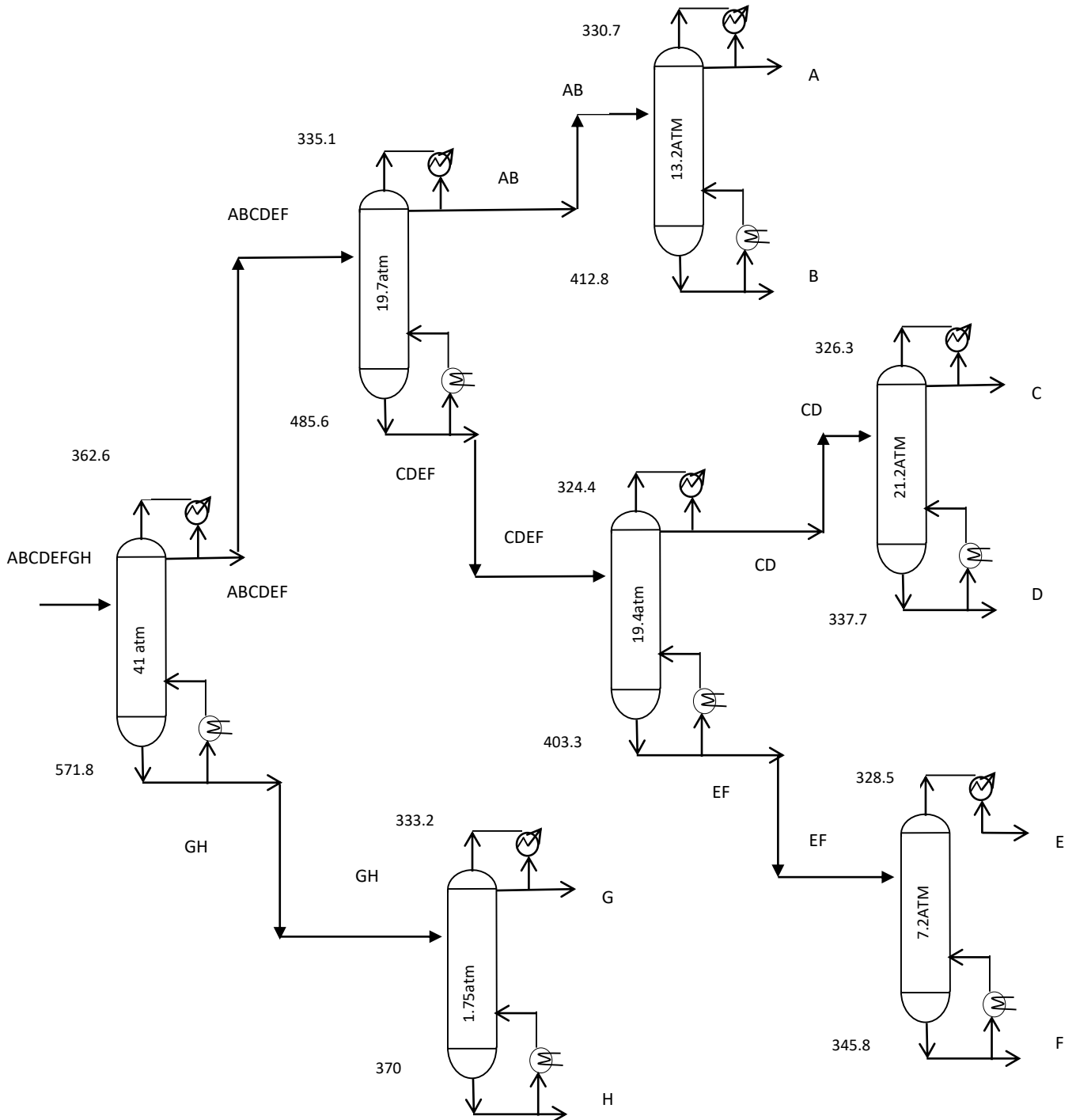
Figure 5 Flow sheet of the separation sequence for case study 2
