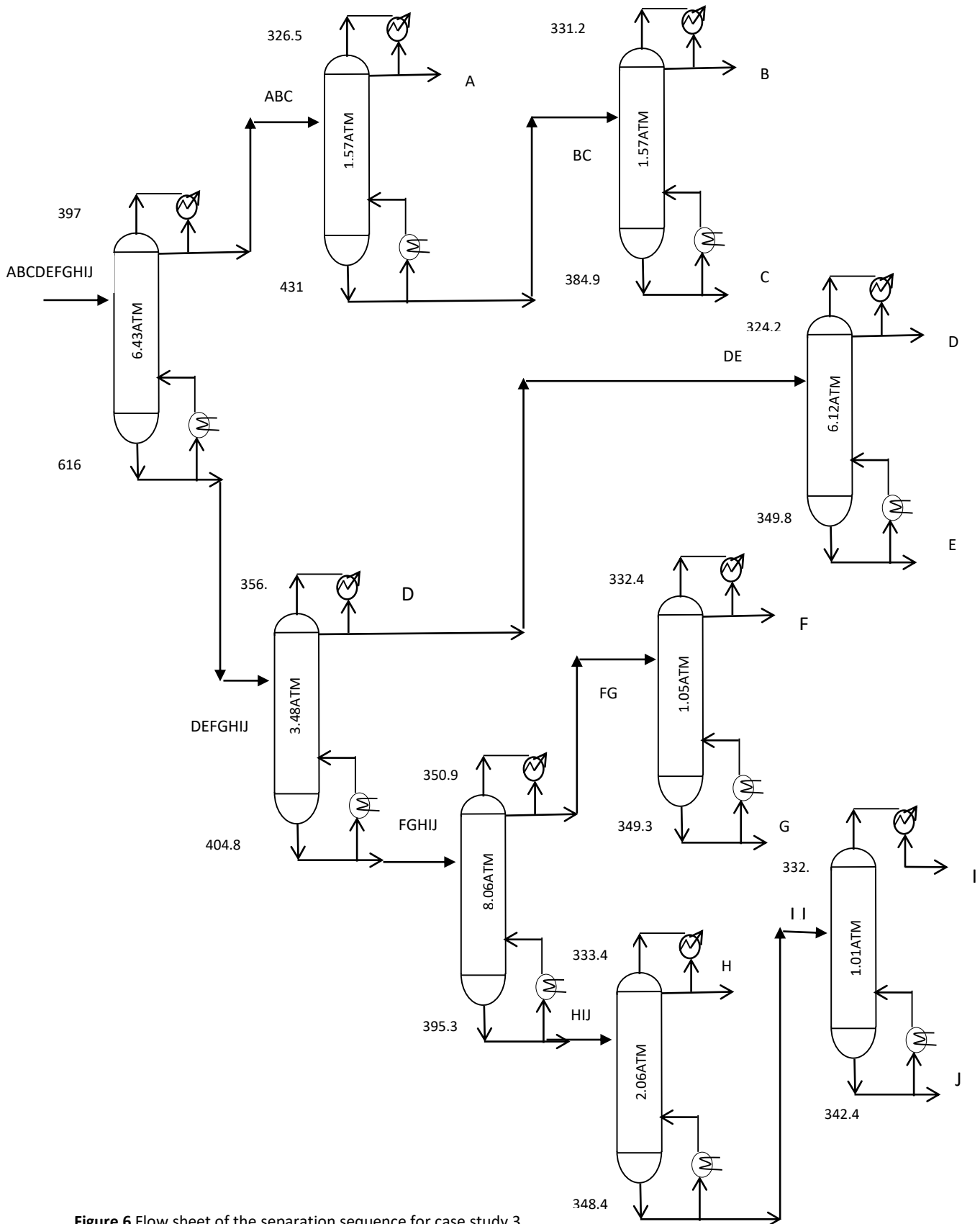
Figure 6 Flow sheet of the separation sequence for case study 3
