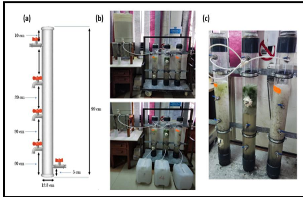
Fig. 3. MBBR experimental system for ammonia removal (a: Schematic Diagram for column dimensions; b: Column technique for biological treatment MBBR, and c: Applied acrylic column (Acrylic is a transparent plastic material with outstanding strength, stiffness and optical clarity))
