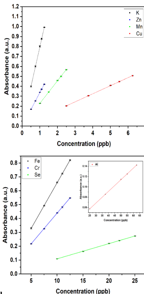
Figure 1. On the first calibration curves of K, Zn, Mn, and Cu. On the second calibration curves of Fe, Cr, Se, and Al.
