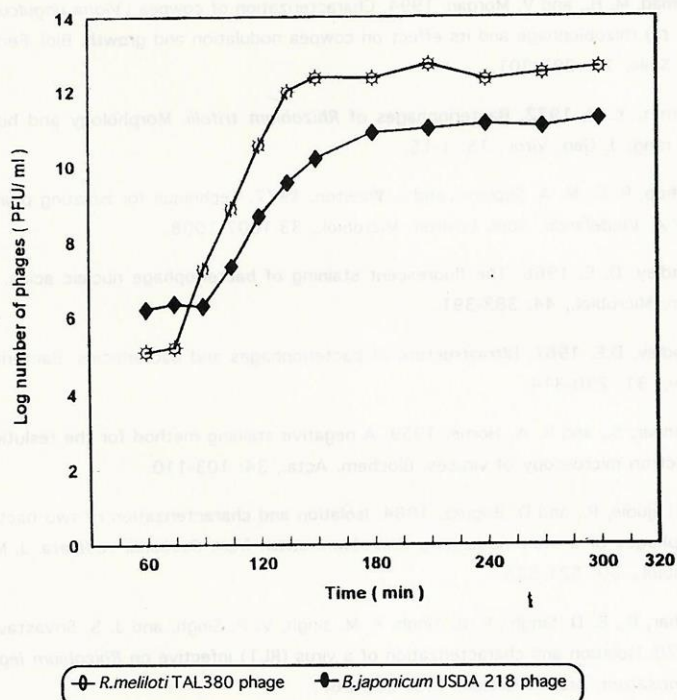
Fig.5. One-step growth experiment of R. meliloti TAL 380 and B. japonicum USDA 218 phages.
