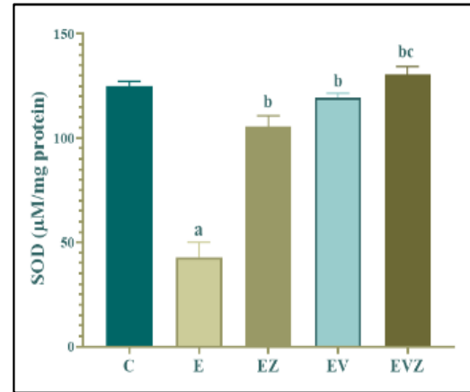
Fig. 4. SOD activity in different examined mice groups. Each value represents the mean \pm SE (n=6) [a: significant from control (P<0.05), b: significant from E (P<0.05), c: significant from EV (P<0.05); and d: significant from EZ (P<0.05)]
