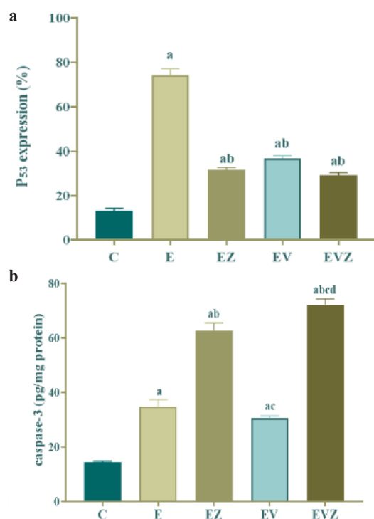
Fig. 7. P53 and Caspase-3 levels in different examined mice groups. Each value represents the
