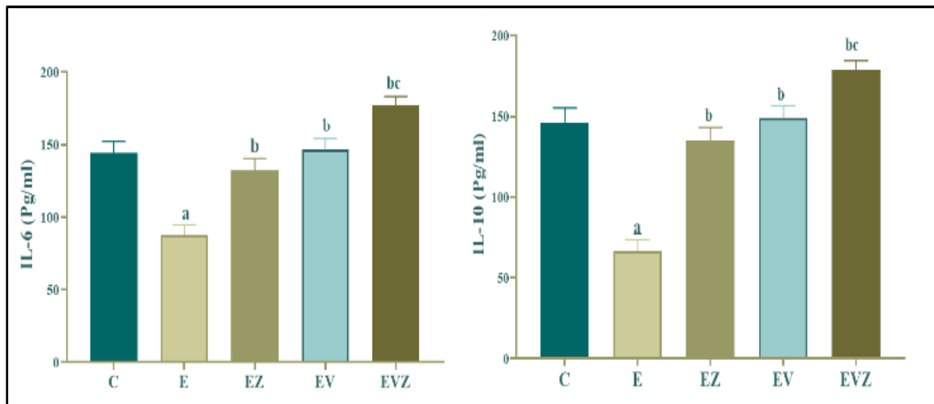
Fig. 5. a) IL-6 level in different estimated groups. b) IL-10 level in different estimated groups [Each value represents the mean \pm SE (n=6). a: significant from control (P<0.05), b: significant from E (P<0.05), c: significant from EV (p<0.05); and d: significant from EZ (P<0.05)]
