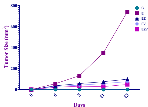
Fig. 1. Effect of irradiated tumor cell lysate vaccine and or ZnONPs on tumor size (mm 3 )
