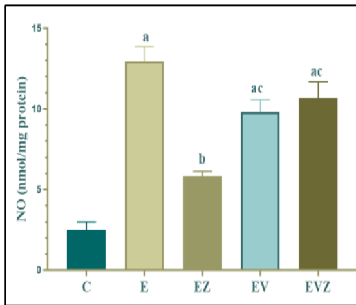
Fig. 3. NO level in different tested groups. Each value represents the mean \pm SE (n=6) [a: significant from control (P<0.05), b: significant from E (p<0.05), c: significant from EV (P<0.05); and d: significant from EZ (P<0.05)]
