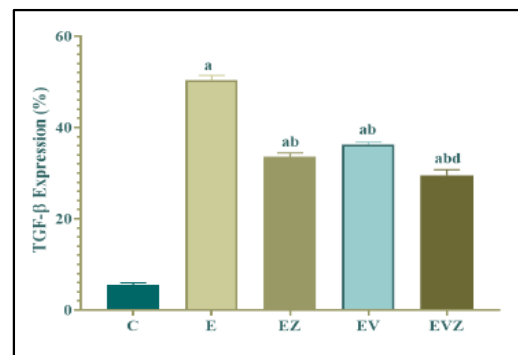
Fig. 6. TGF \beta m-RNA gene expression in different examined mice groups. Each value represents the mean \pm SE (n=6) [a: significant from
