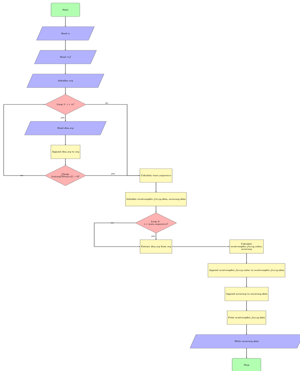
Figure 2. The flow chart of the proposed algorithm
