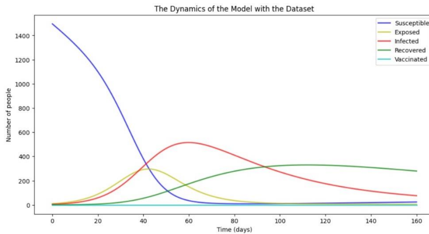
Figure 3. Population dynamics in Ghana, including susceptible, exposed, infected, vaccinated, and recovered states, as experienced across time. Various shades of hue denote distinct demographics: The colors blue, yellow, red, cyan, and green represent different stages of infection and recovery.
