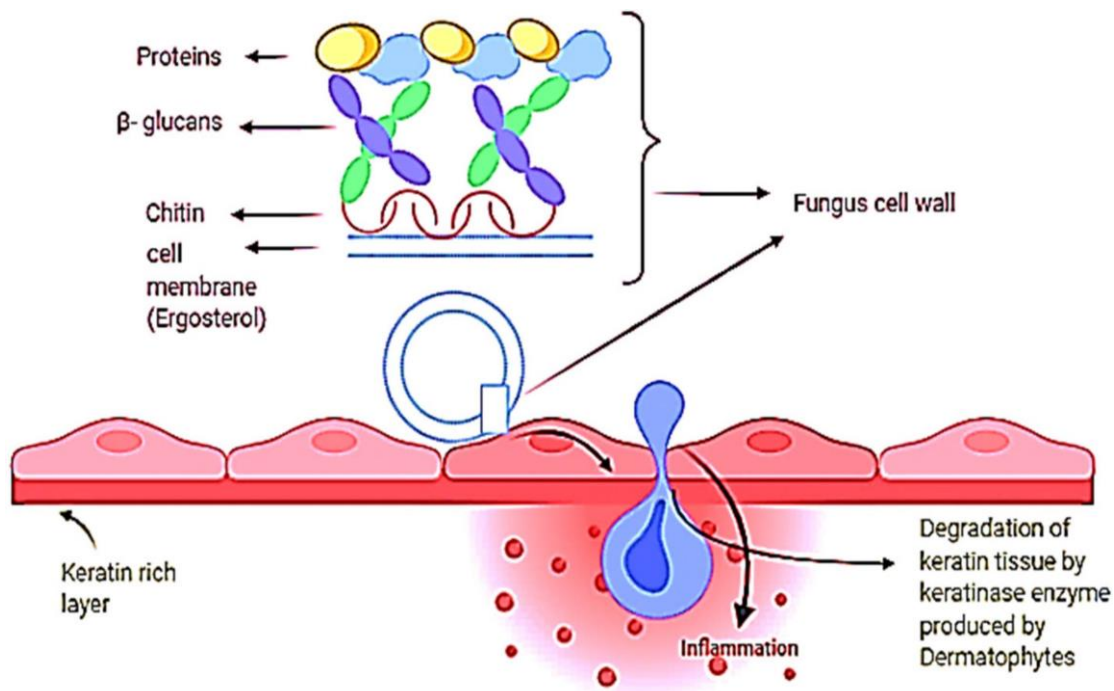
Figure 1. Schematic illustration of Tinea Pedis pathophysiology (dermatophytosis; Figure from Navkiranjeet et al, 2021 [4]).
