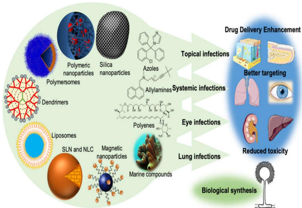
Figure 3. Advanced antifungal delivery systems (Figure from Sousa et al, 2020 [15]).
