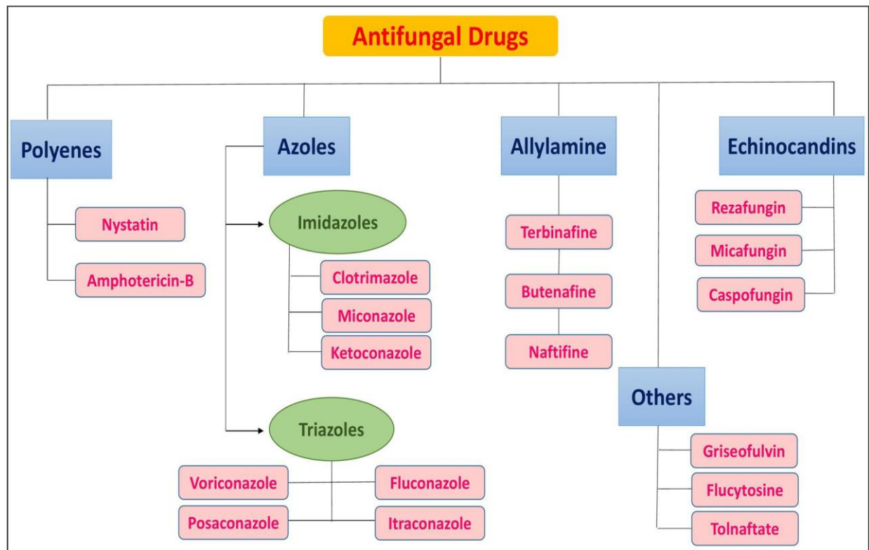
Figure 2. Schematic categorization of antifungals that can be used for tinea pedis treatment
