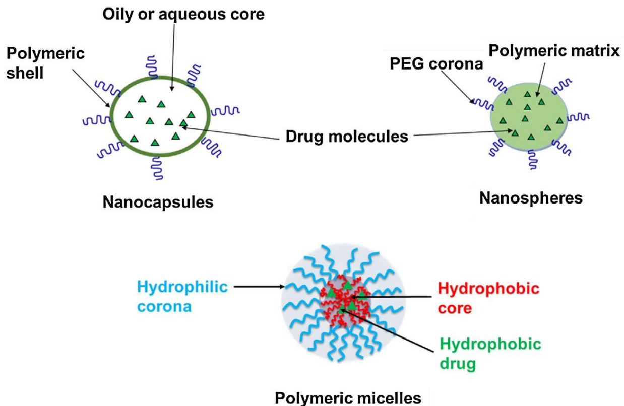
Figure 6. Types of polymeric nanoparticles used for antifungal delivery (Figure from Soliman et al, 2017 [6]).
