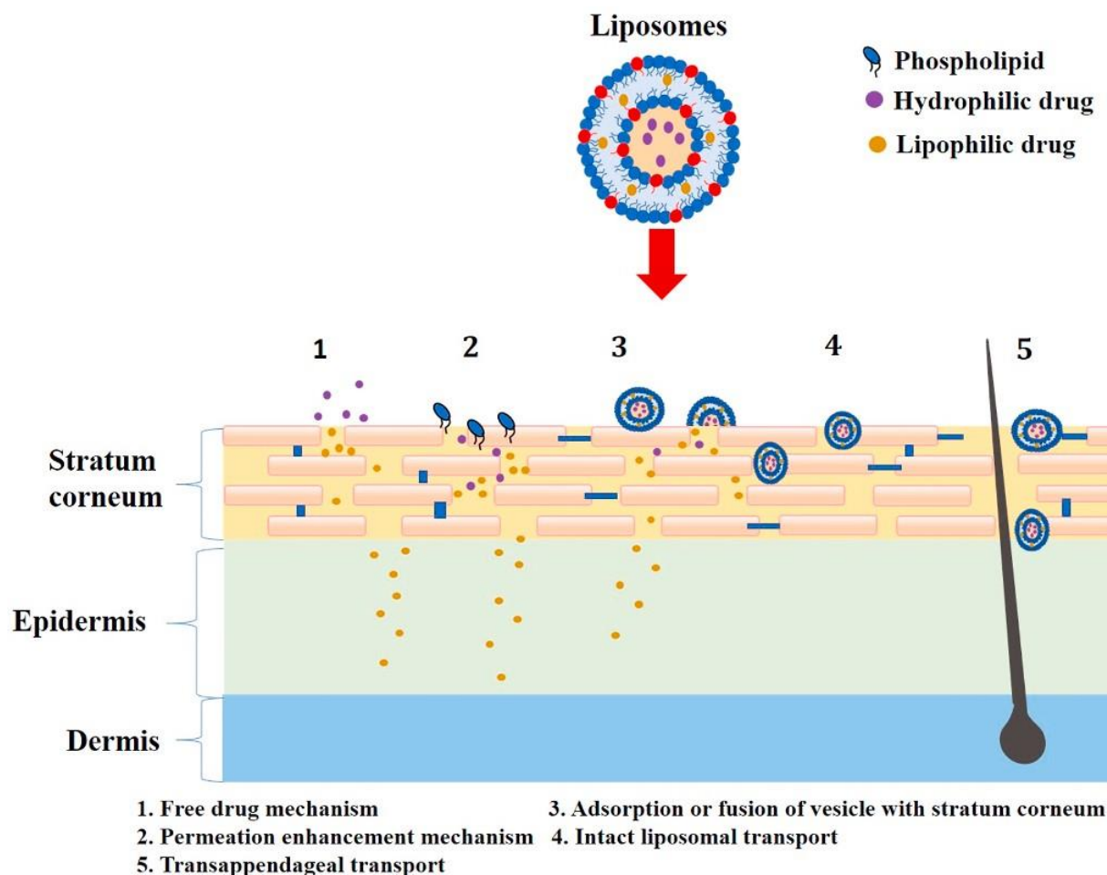
Figure 5. Mechanism of skin permeation of liposomes (Figure from Nene et al, 2021 [17]).
