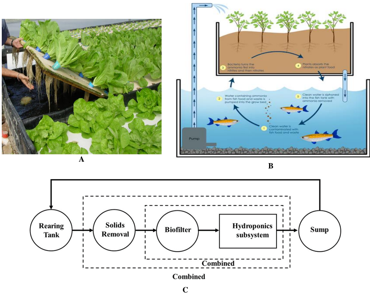
Figure 2 A: Hydroponics, B: Aquaponic system, and C: Aquaponic system layout [32].
