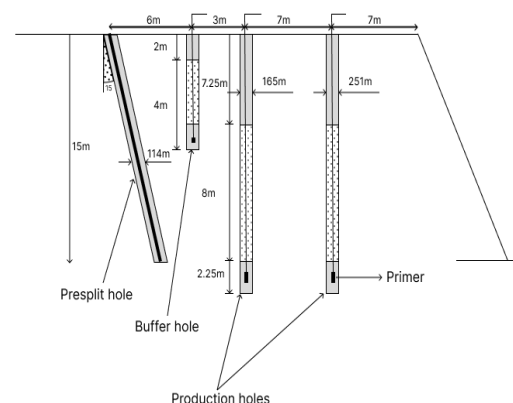
Figure 1 Schematic diagram of drilling profile (modified after [10])
