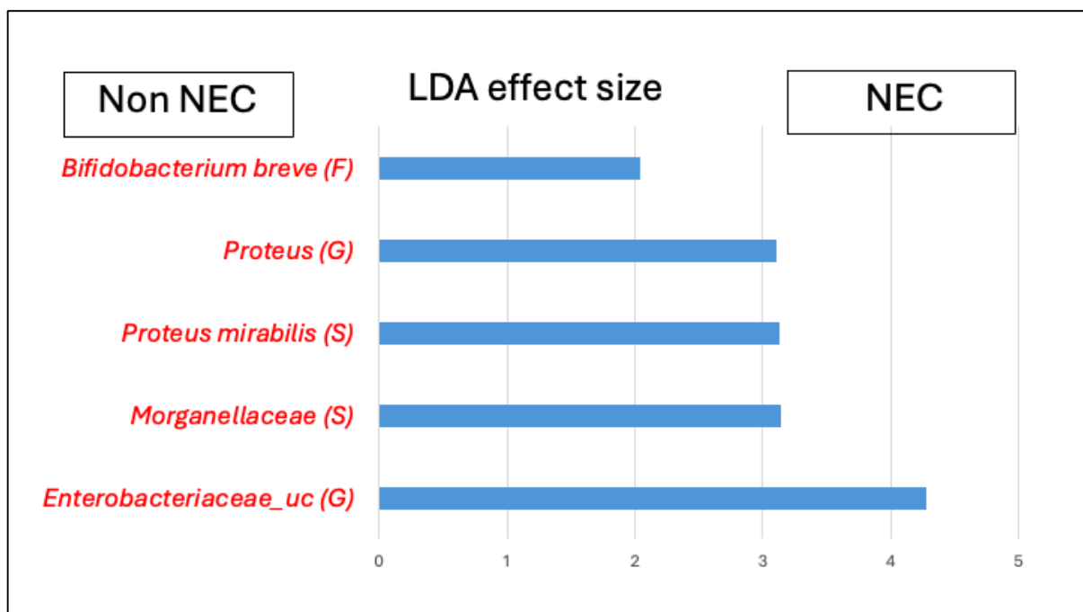
Figure 4. LDA (Linear discriminant analysis) score between NEC and non-NEC group calculated based upon the Lefse analysis describing the effect in the significantly different taxa in each group.
