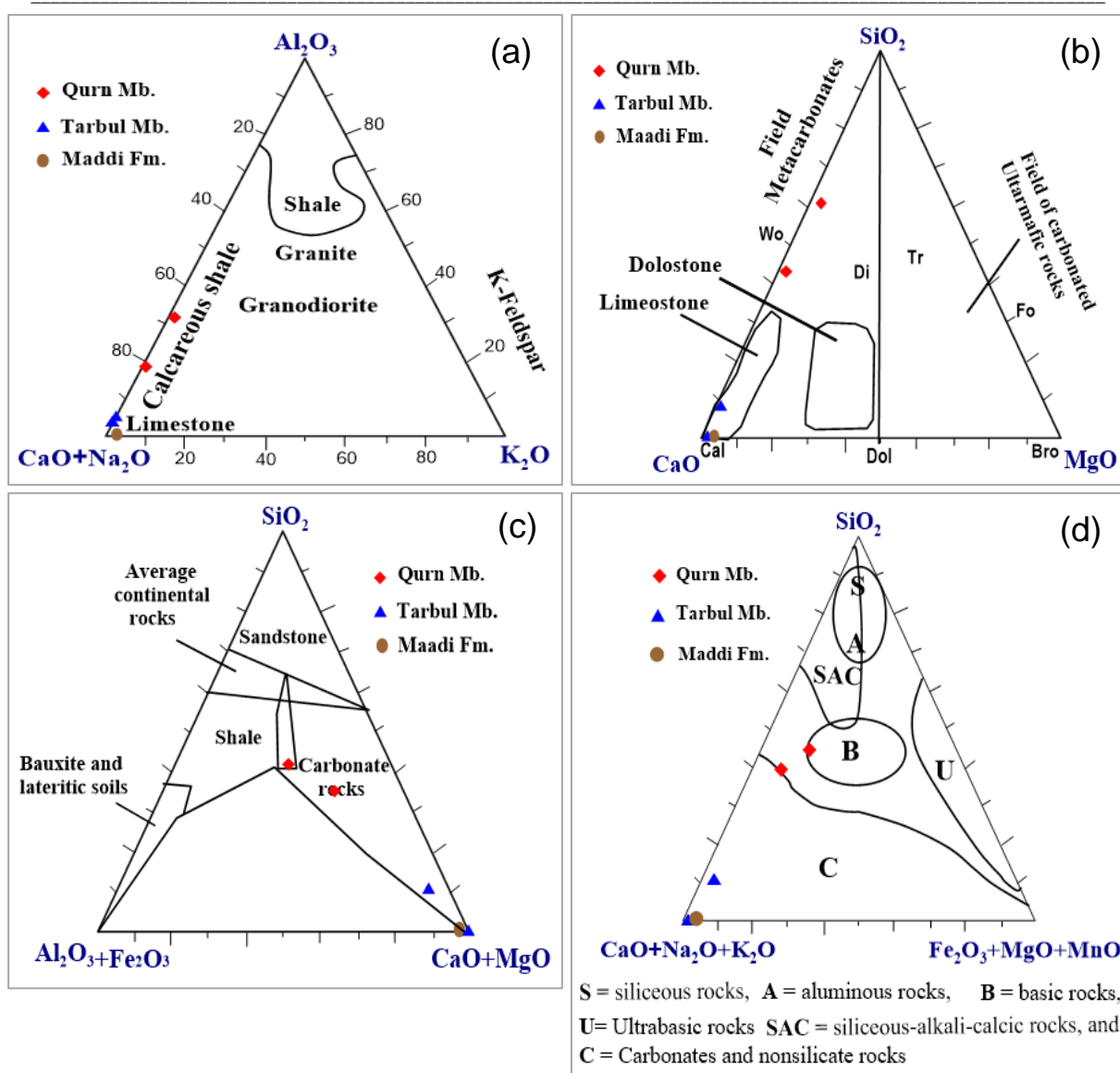
Fig. 7 (a). Ternary diagram (Hutcheon, 1998) between Al_2O_3 - (CaO+Na_2O) - (K_2O) for the studied samples, (b) Ternary diagram between SiO_2 - CaO - (MgO) (Winter, 2001) for the studied samples, (c) Ternary diagram between SiO_2 - (Al_2O_3+Fe_2O_3) - (CaO+MgO) (Mason & Moor, 1982) for the studied samples, and (d) Ternary diagram between SiO_2 - (CaO+Na_2O+K_2O) - (Fe_2O_3+MgO+MnO) (Raymond, 1995) for the studied samples.
