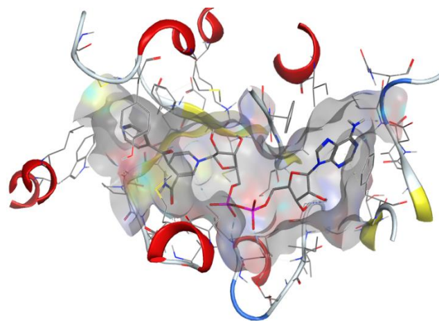
Fig. 7: (a) 2D and (b) 3D binding modes of isonicotinoyl-NADH complex inside InhA active site (PDB:1zid).
