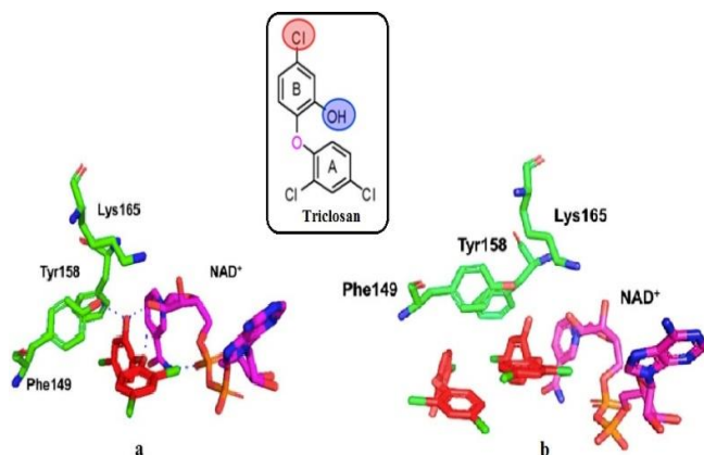
Fig. 8: (a) Representation of the key interactions of triclosan (red) bound to the InhA binding site & (b) A view of two molecules of triclosan (red) within the active site. NAD + (magenta) and binding site residues (green).
