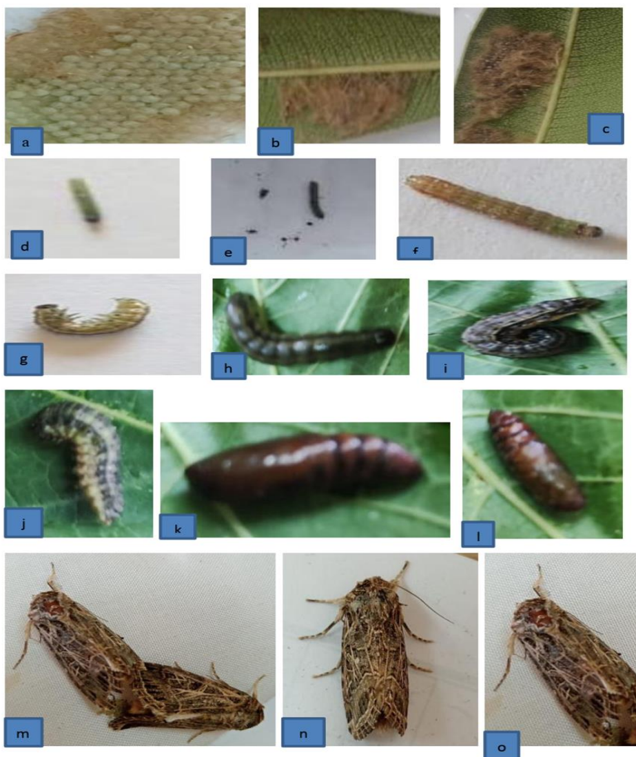
Fig. 1. Stages of S. frugiperda ; (a) eggs, (b) egg starting to hatch (c) newly hatched larvae, (d) 1 st instar larva, (e) 2 nd instar larva, (f) 3 rd instar larva, (g) 4 th instar larva, (h) 5 th instar larva, (i) 6 th instar larva (j) Prepupae, (k) pupae male, (l) pupae female, (m) mating, (n) adult of male and (o) adult of female.
