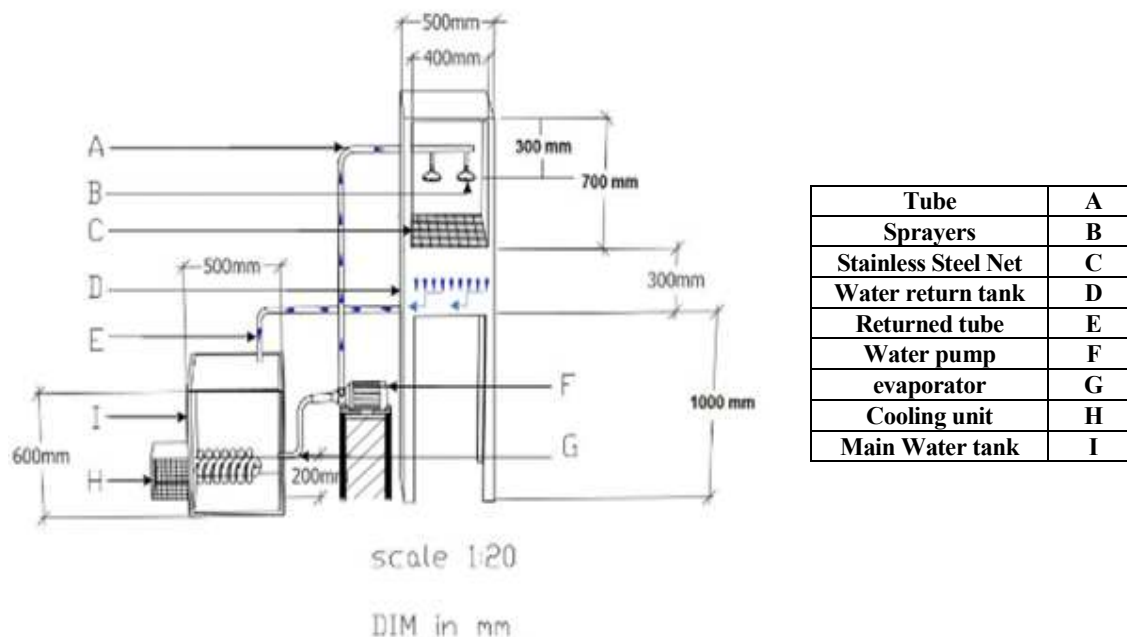
Fig. 1. Schematic diagram for the portable pre-cooling unit
