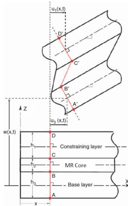
Figure (3): The undeformed (dashed line) and the deformed (Solid line) configurations of a three-layer sandwich beam under lateral loading
