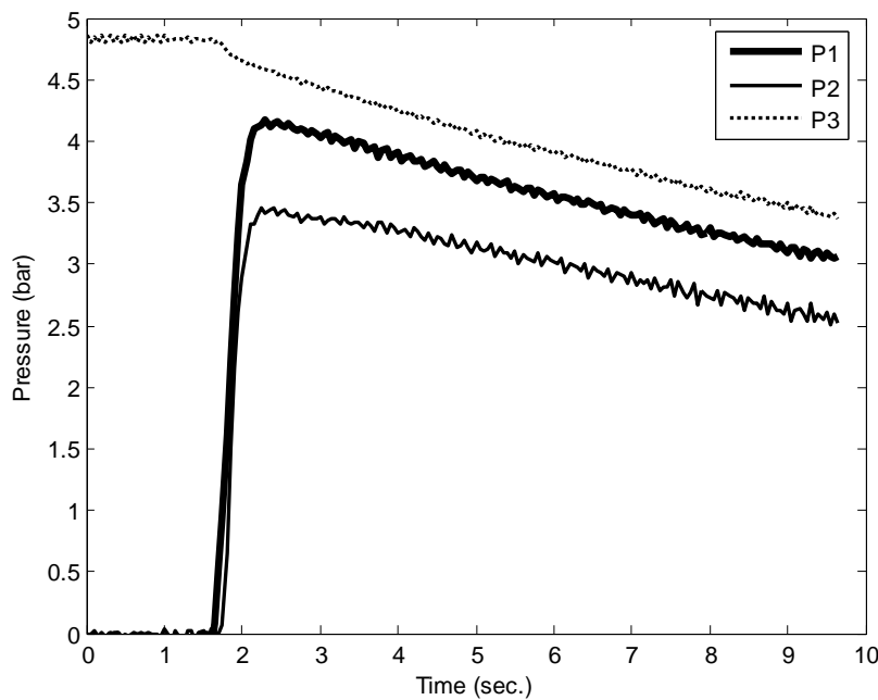
Figure (10): Effect of leak in air brake pressure.
