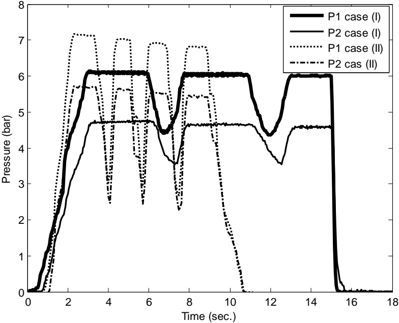
Figure (7): Air line brake pressure at half load in two cases at variable pedal travel
