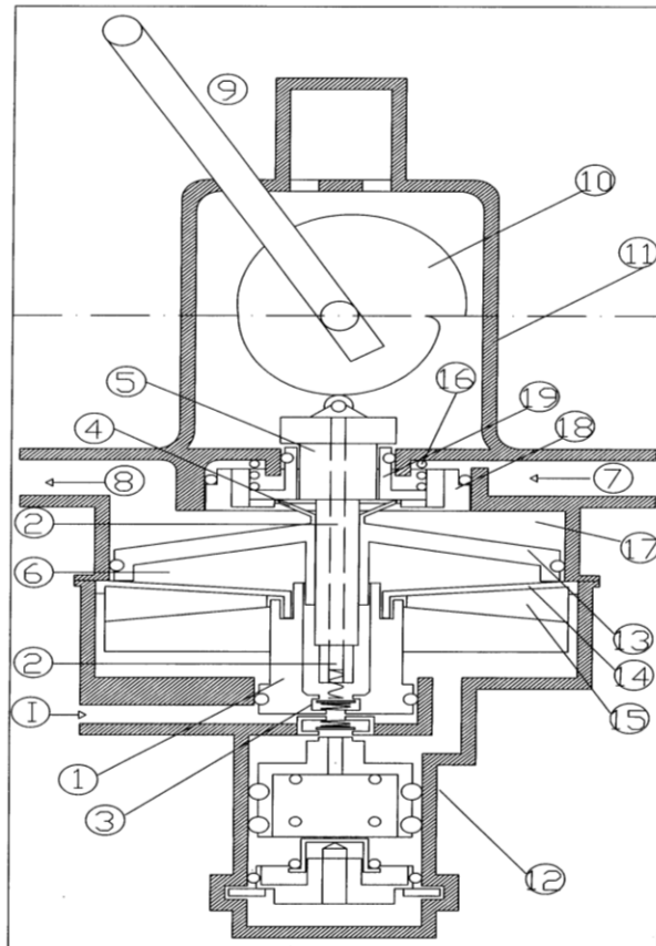
Figure (1): Load sensing relay valve main parts [11].
