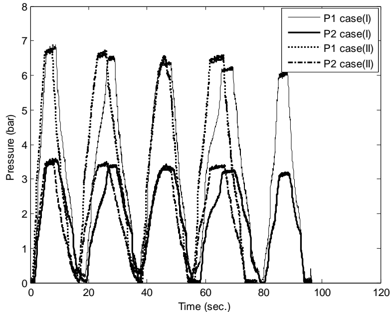
Figure (8): Air line brake pressure at no- load in two cases at variable pedal travel
