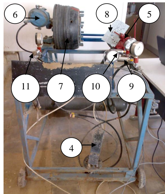
Figure (3-b): Data Acquisition System Components [DAQ]
