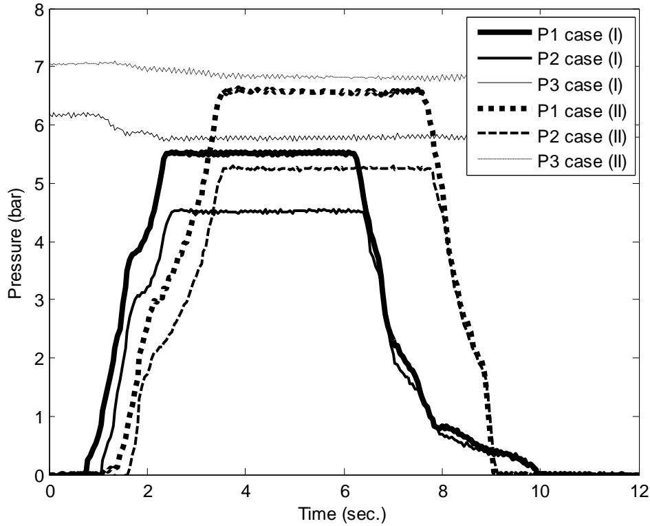
Figure (4): Air line brake pressure at half-load in two cases
