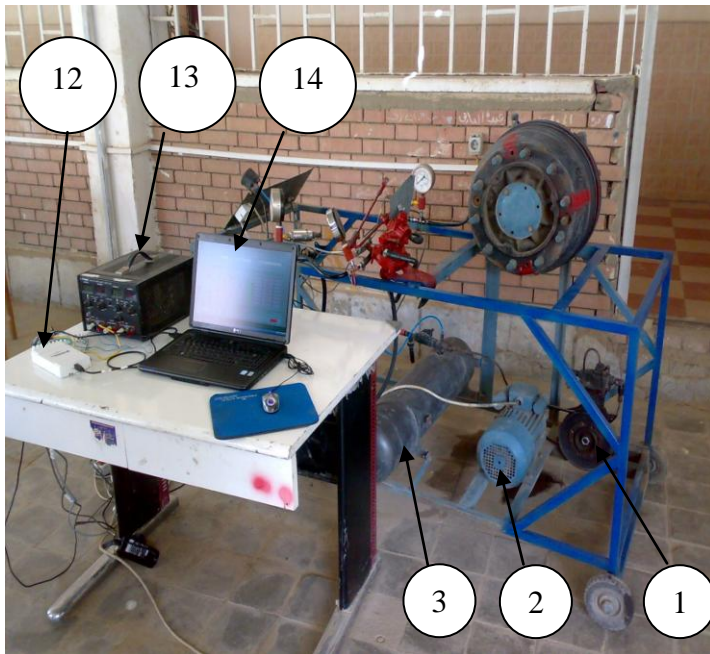
Figure (3-a): Air brake system components
