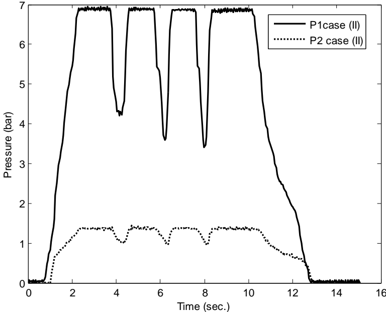
Figure (6): Air line brake pressure at (1/3) load in case (II) at variable pedal travel
