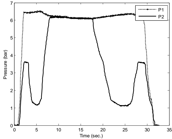
Figure (9): Wheel chamber air brake pressure at different loading conditions.
