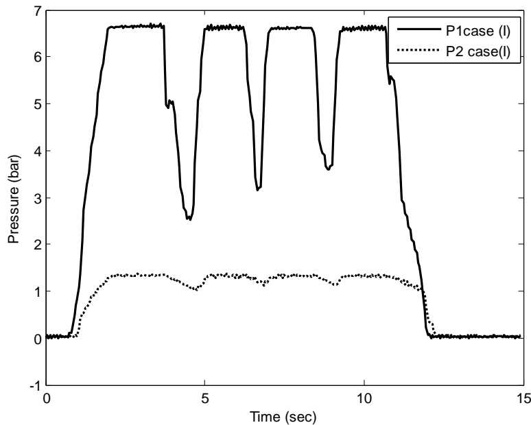
Figure (5): Air line brake pressure at (1/3) load in case (I) at variable pedal travel
