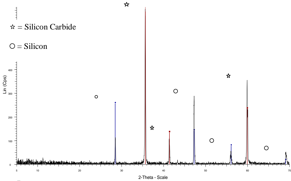
Fig. (3b) XRD patterns of the Si/SiC 8 Wt.% bodies fired at 1500°C
