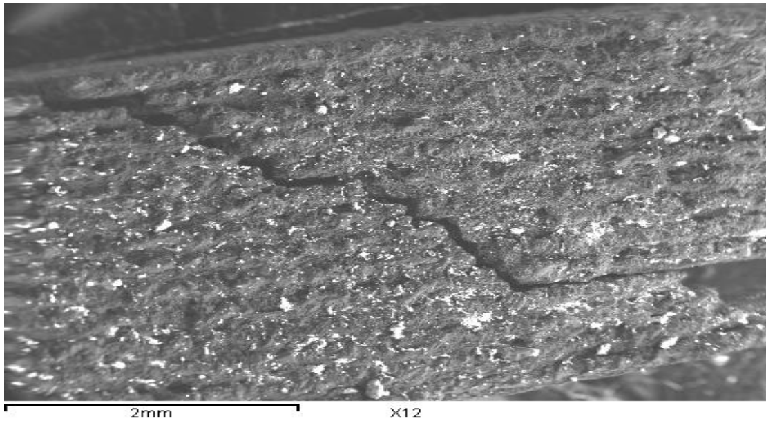
Fig. (7) Crack deflection occurs at the Si/SiC-Si/SiC interface.
