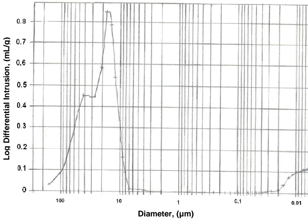
Fig.(6a) The analysis of pore size distribution carried out for the carbon substrate
