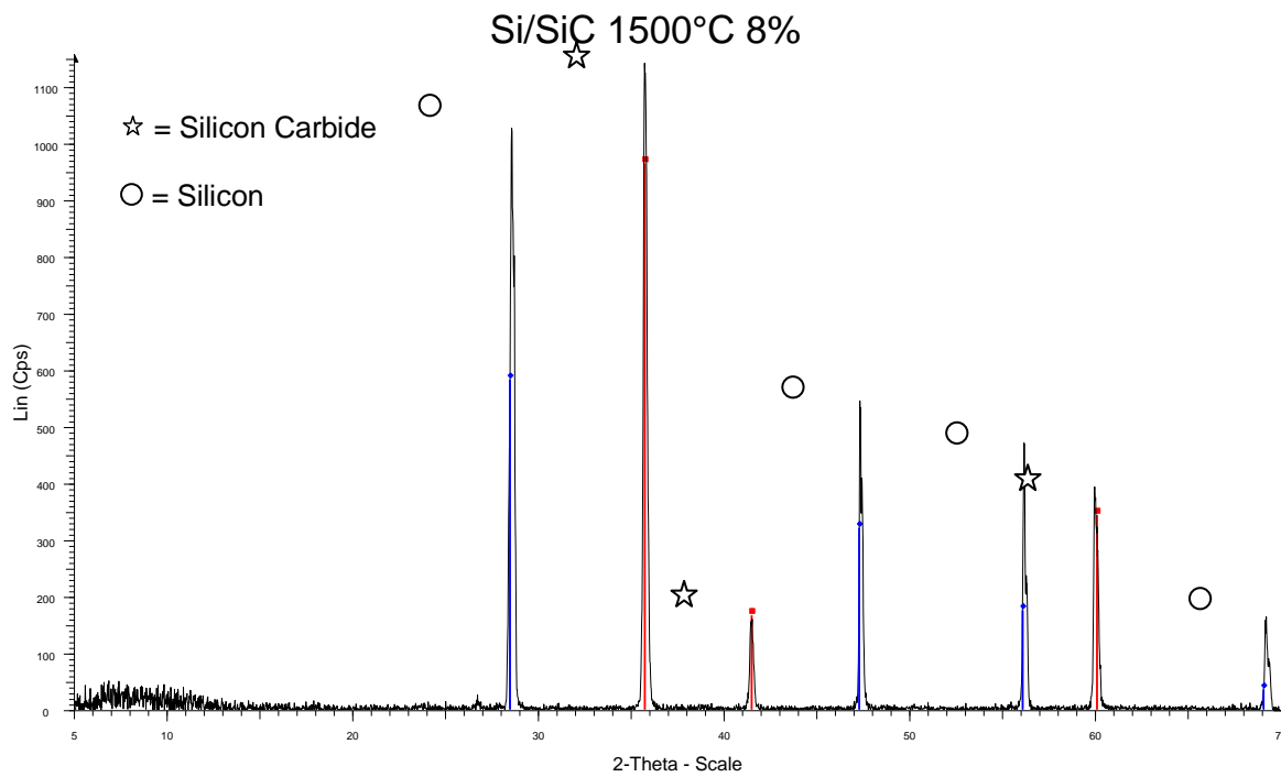
Fig. (3a) XRD patterns of the Si/SiC 8 Wt.% bodies fired at 1500°C
