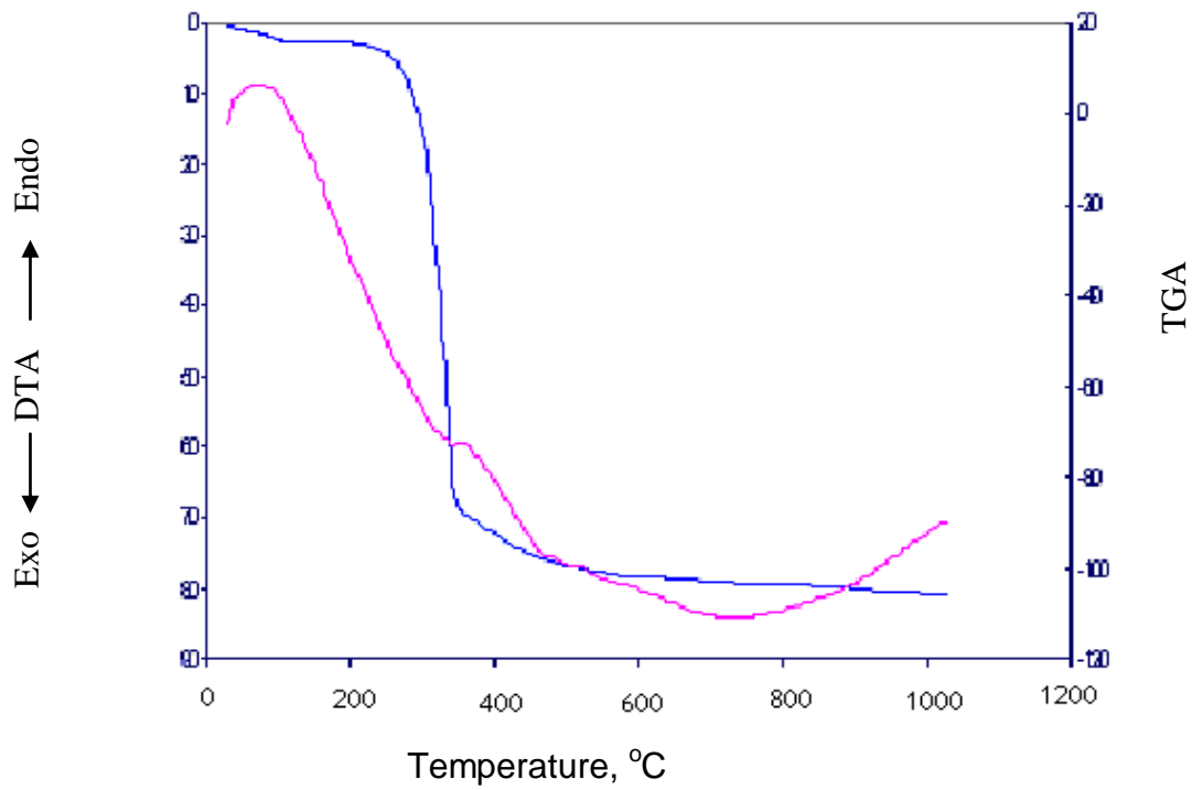
Figure (2) DTA and TG curves of the raw textile
