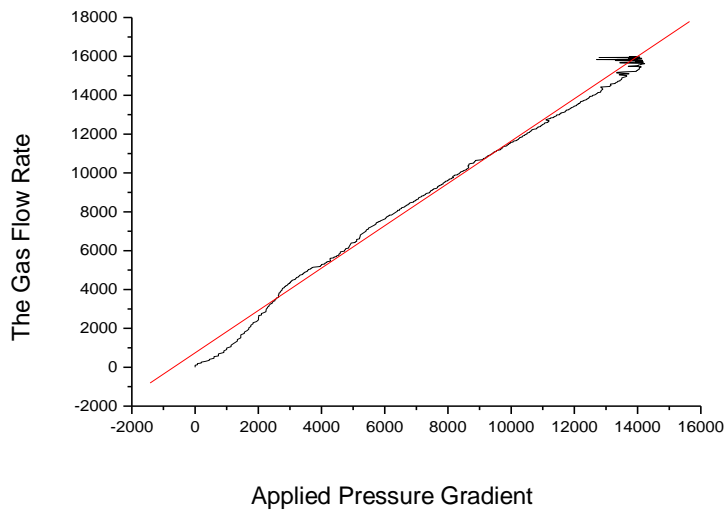
Fig. (5): The gas permeability of the Si/SiC composites containing 4.5 wt % Si.
