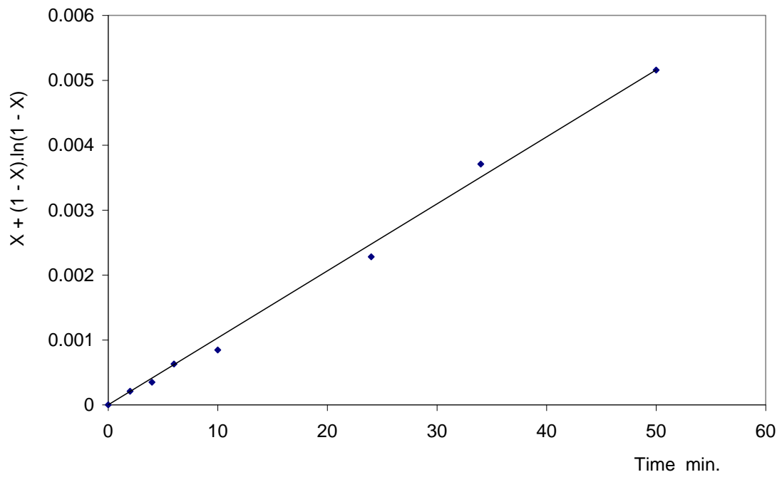
Fig (10): Plot of f(X) against oxidation time for diffusion controlled reaction
