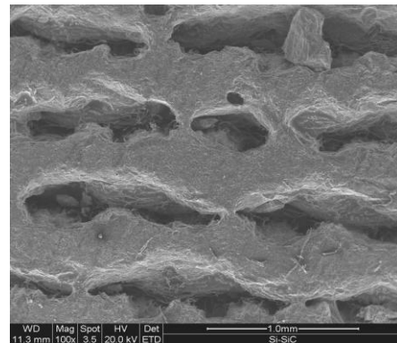
Fig. (4b) cross section SEM micrograph of laminated Si/SiC composite fired at 1500°C showing necks between the stacked layers.
