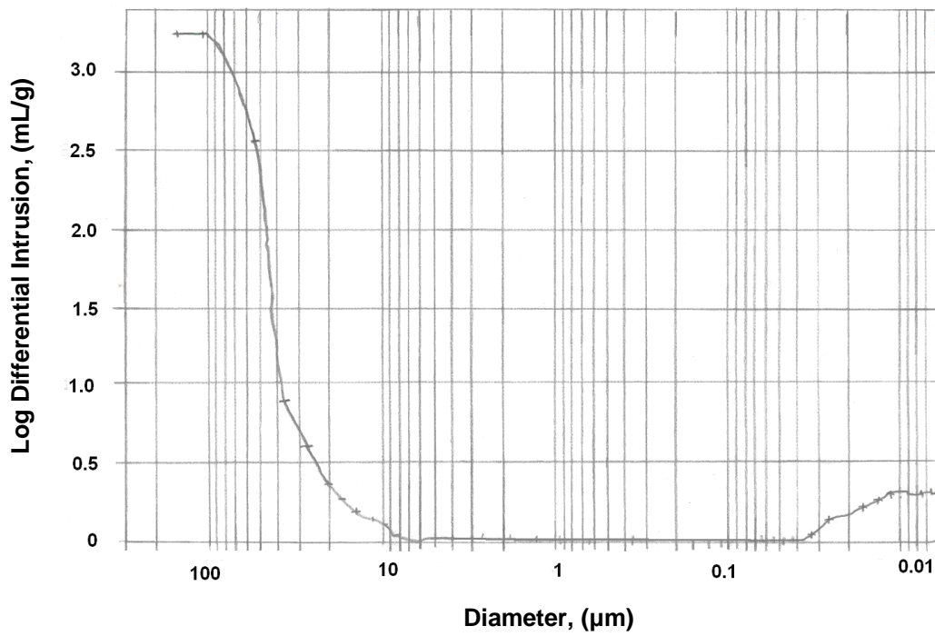
Fig.(6b) The analysis of pore size distribution carried out for the Si/SiC composite
