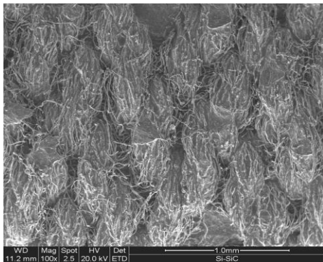
Fig. (4a) SEM micrograph of a single layer of laminated Si/SiC composite fired at 1500°C showing retention of the native fabric architecture
