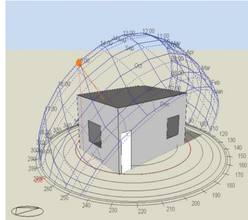
Fig(15)_ Office room build on design building Showing north direction .
