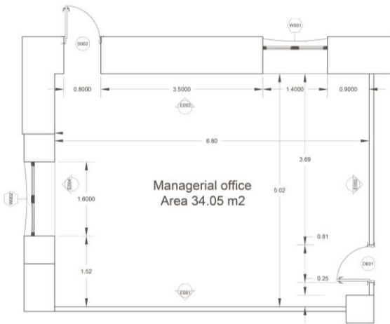
Fig (14) _Manager office plan used in the experiment.
