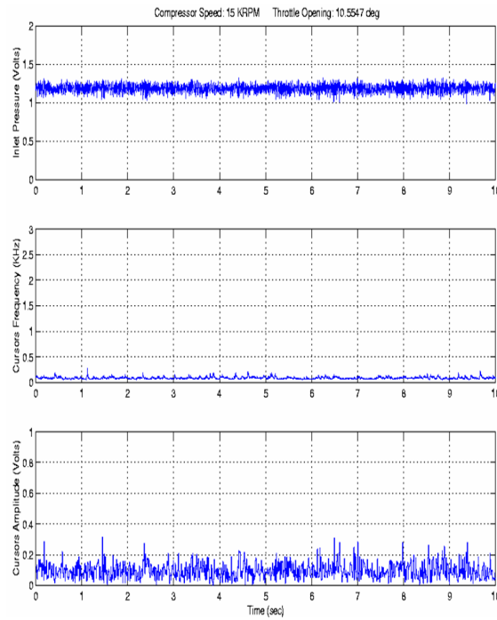
Figure 6. High Back Pressure Nearing Surge, 15 KRPM
