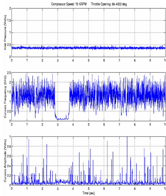
Figure 4. Low Back Pressure, 15 KRPM
