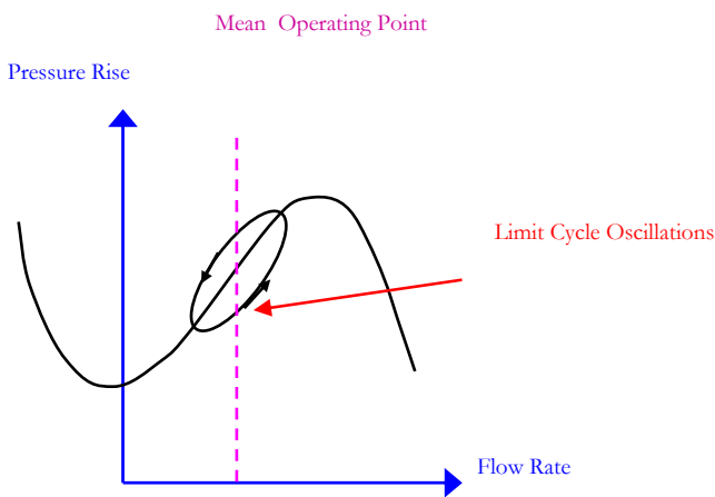
Figure 3. a. Mild Surge
