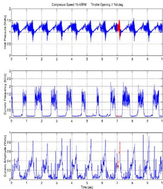
Figure 5. Uncontrolled Surge, 15 KRPM
