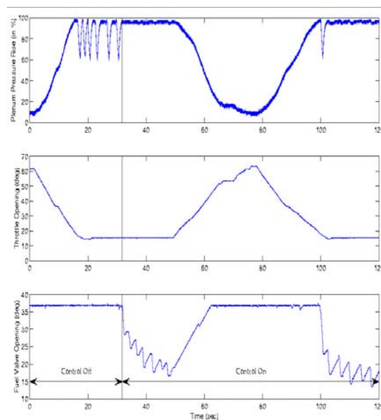
Figure 9. The response of the compression system with Using Fuel Valve Actuation
