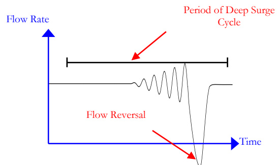
Figure 3.d. Deep Surge of the Flow Rate
