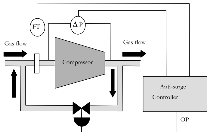
Figure 1. The Compression System
