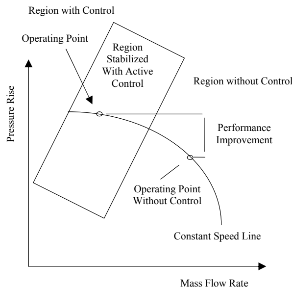
Fig. 2. Compressor Performance Characteristic Map
