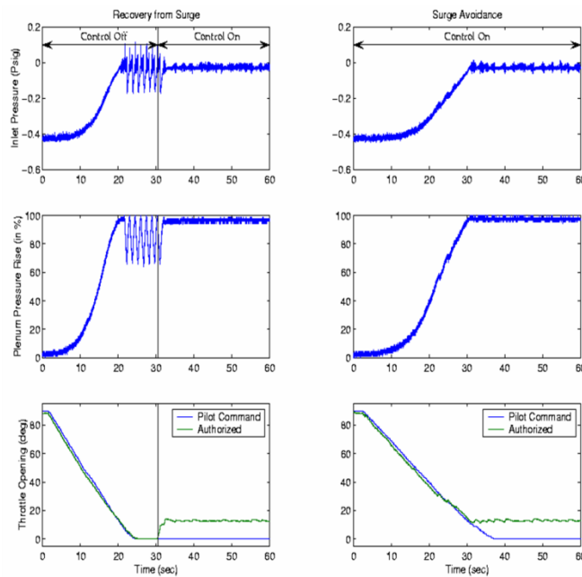
Figure 8. The response of the compression system with control of surge using fuzzy logic Control
