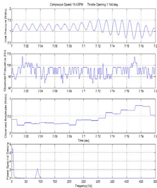
Figure 7. Uncontrolled Surge, 15 KRPM
