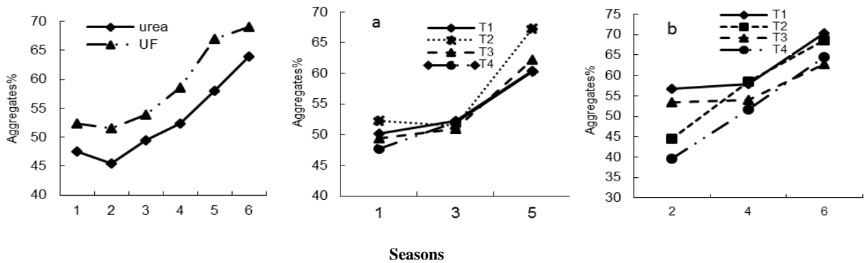
Fig. (13): Effect of urea & UF fertilizers, sunflower/cowpea (a) and wheat/peas (b) intercroops configurations on averages of total wet stable aggregates%.
