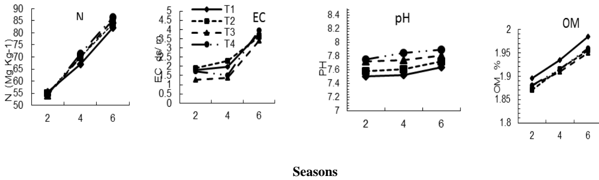
Fig. (11): Effect of wheat/peas intercroops configurations on available-N, EC, pH and OM
