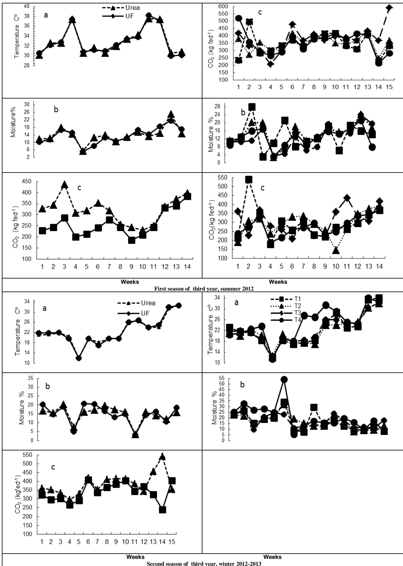
Fig.(4): Soil temperature (a), soil moisture (b) and soil emitted CO 2 (c) at different treatments during third year of 3 successive years
