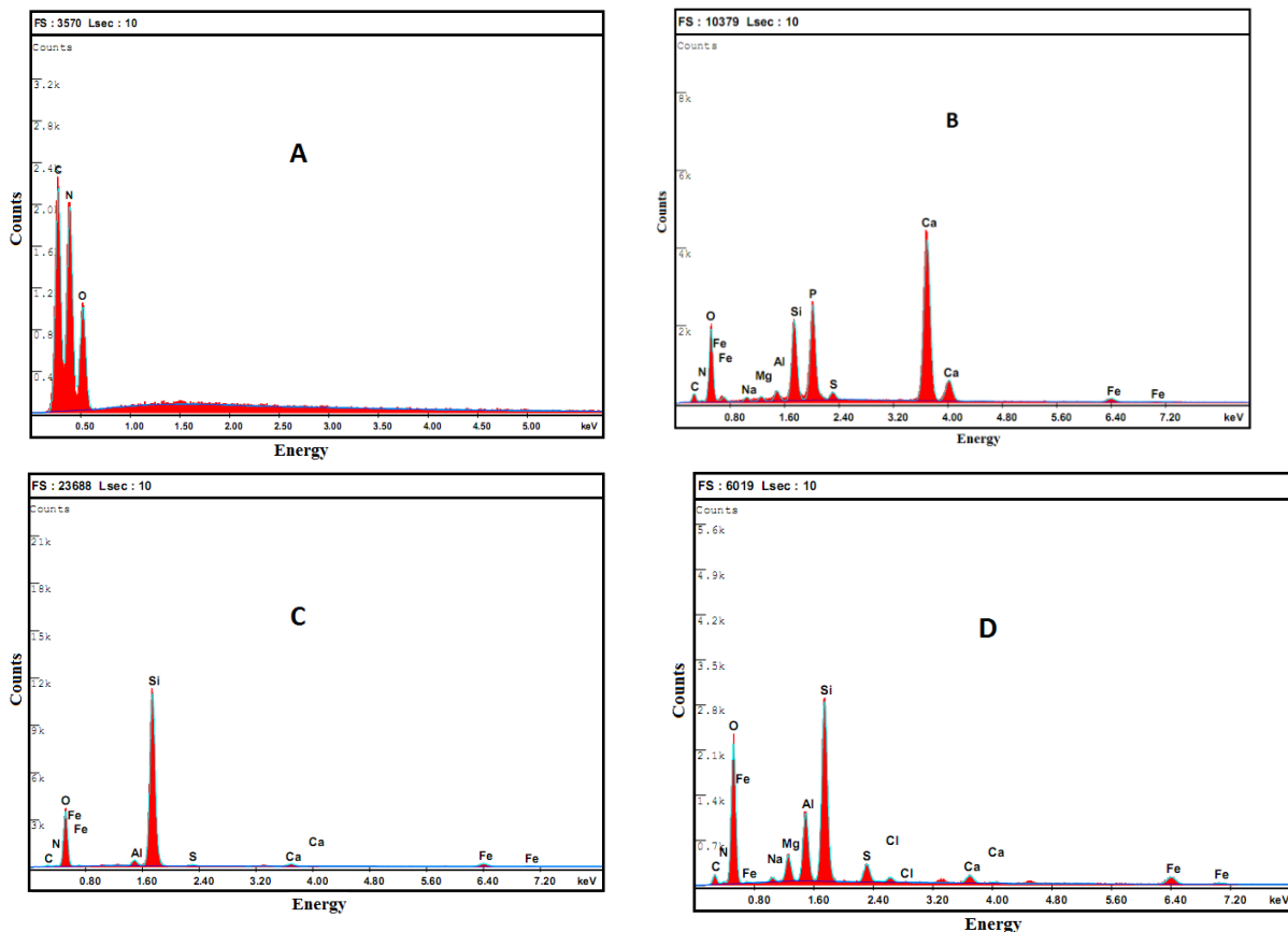
Fig. 4. EDX Diagram of (UCU) (A), (PCU) (B), (SiCU) (C) and (BCU) (D) Materials.
