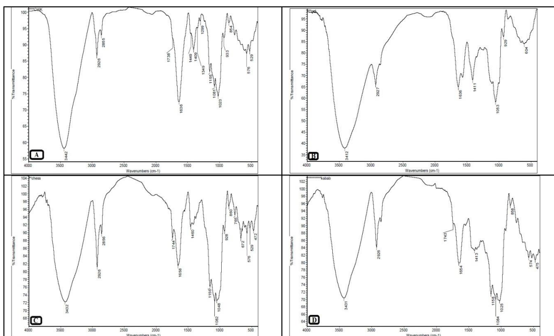
Figure (1): The FT-IR spectra of studied flavoring agents (A- chicken, B- catchup, C- cheese and D- kabab) in the spectral range of 400-4000 \text{cm}^{-1} .
