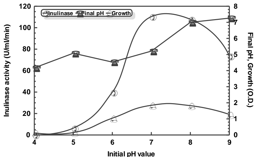
Fig. 2. Effect of medium initial pH on inulinase production by Acetobacter sp.
