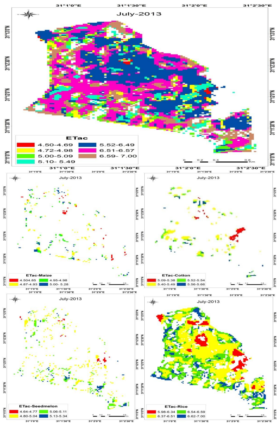
Fig (6): Estimated ET c (mm) for summer crops in July (2013) extracted from Landsat data.
