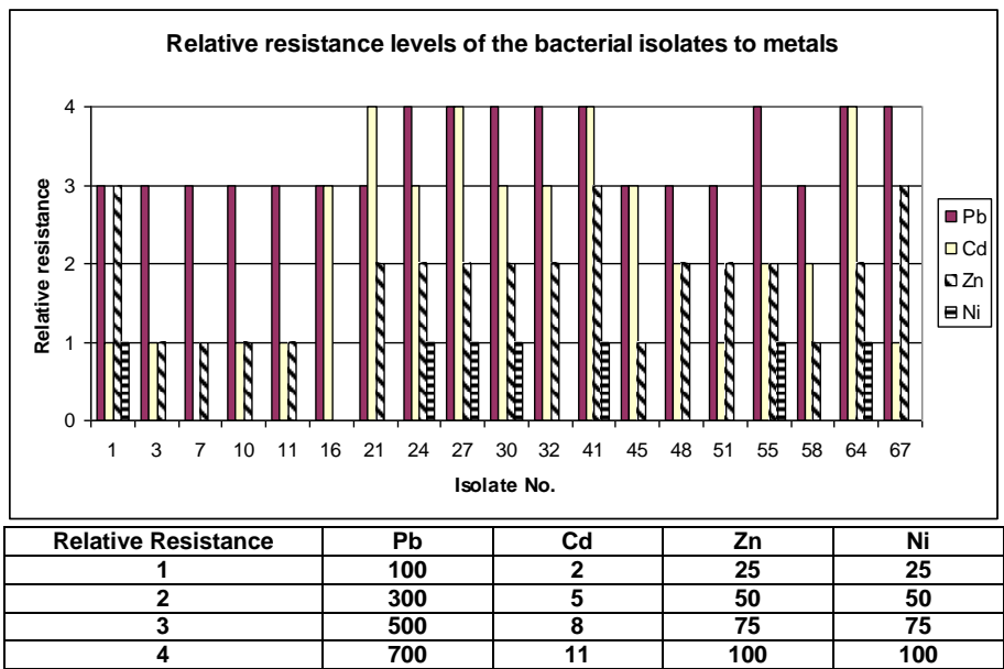
Fig. 3: The relative resistance of the bacterial isolates for the maximum tolerance heavy metal concentrations.
