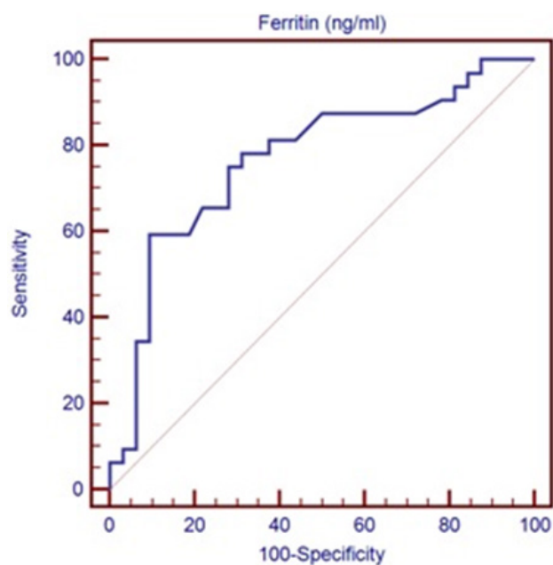
Fig. 1: Receiver operating characteristic curve showing the best cutoff point for serum ferritin level between mothers with asymmetric IUGR neonates and those with AGA, was >18.2 ng/mL.
