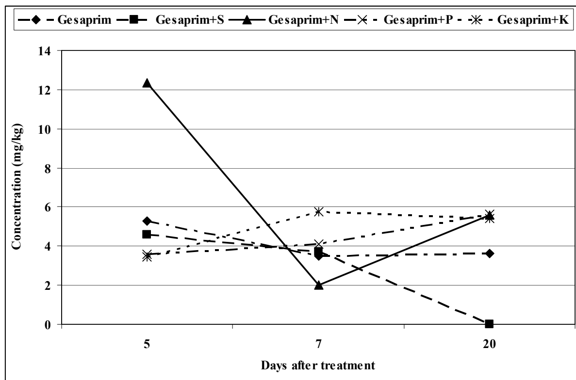
Fig. 1. Residues (mg/kg) of Gesaprim in the soil of maize field
