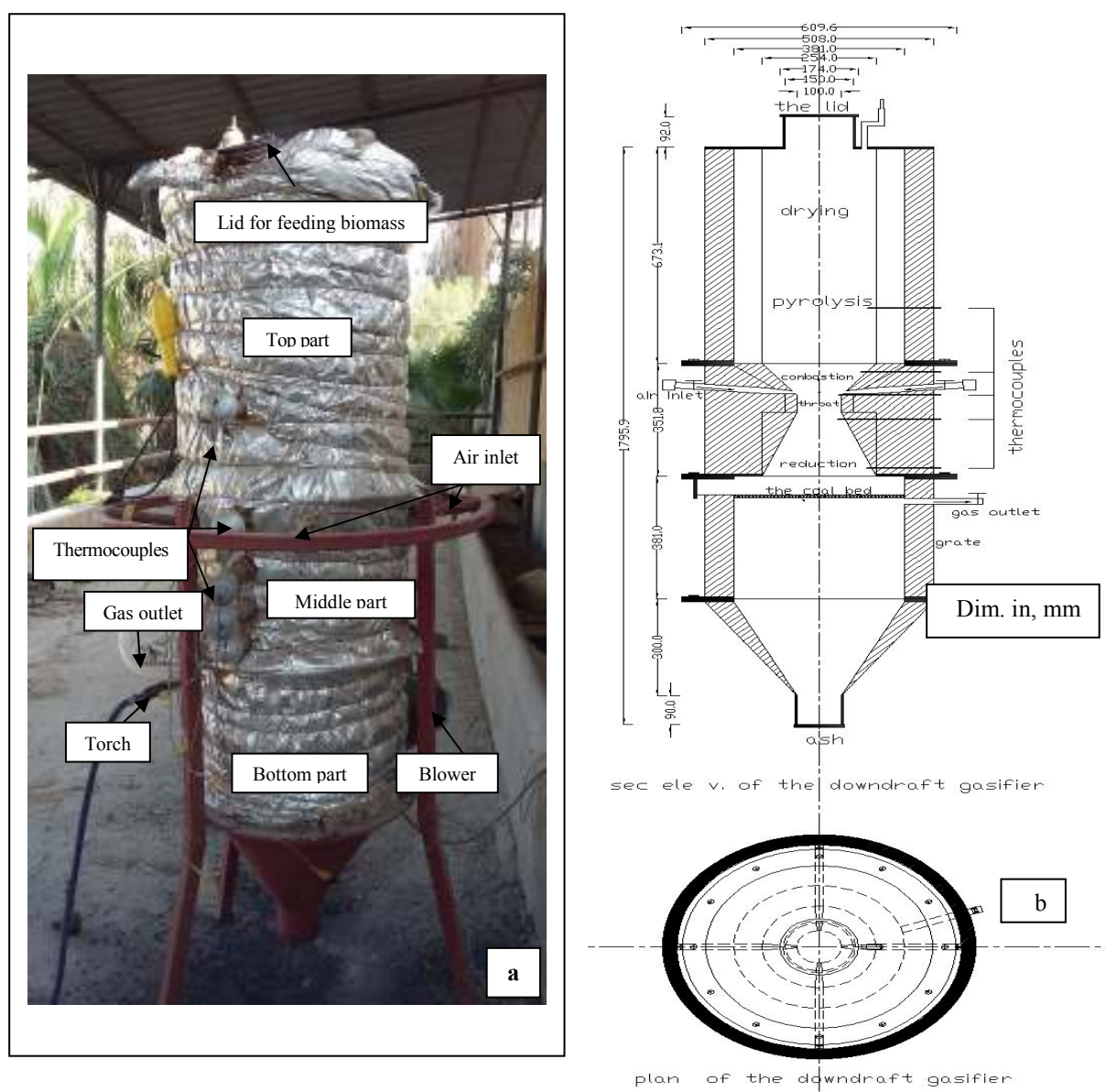
Fig. 1. The gasification unit: a) the prototype fixed bed downdraft gasifier, b) cross sectional and plan views of the gasifier
