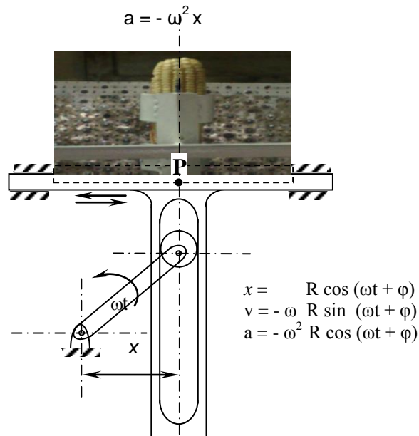
Fig. (2): The prototype layout
