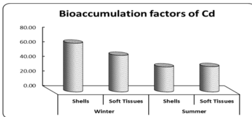
Fig. 3: Bioaccumulation factors of cadmium ion in Patella caerulea (shells and soft tissues) during this study.
