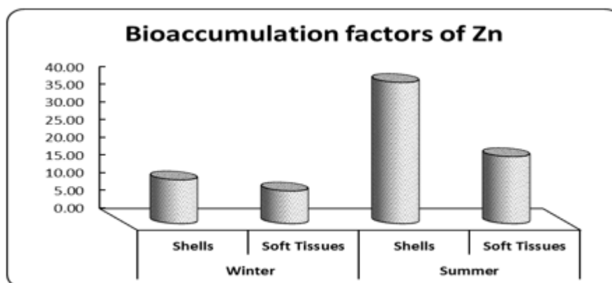
Fig. 21: Bioaccumulation factors of zinc ion in Patella caerulea (shells and soft tissues) during this study.
