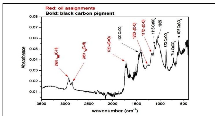
Figure (7) Shows FTIR spectrum of the drying oil medium
