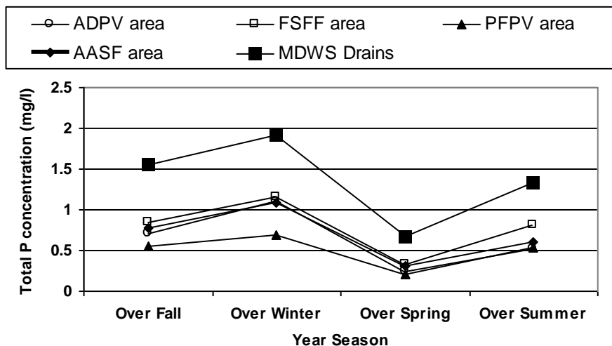
Figure (2): Seasonal means of surface and ground water phosphorus concentrations as affected by different agricultural activities.
