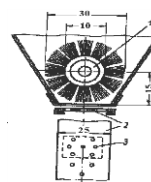
Fig. (7): A brush-type device for sowing small seeds:
