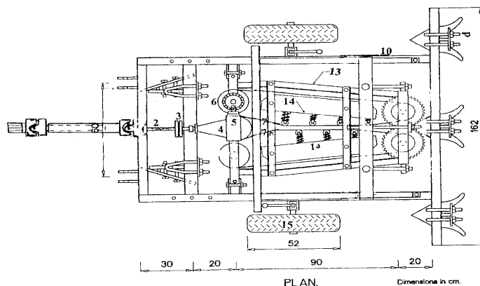
Fig. (5): Sketched of elevation and plan views of the developed planting and harvester sugar beet machine.
