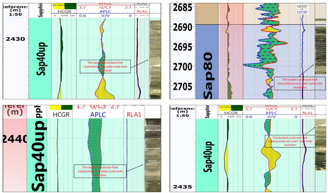
Figure 8. Shows conventional core versus logs at depth (2430m-2704m).
