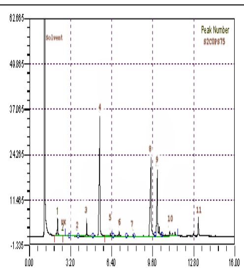
Fig.(2): G. L .C analysis of volatile oil of plant treated with C0 + PS75 2 nd season
