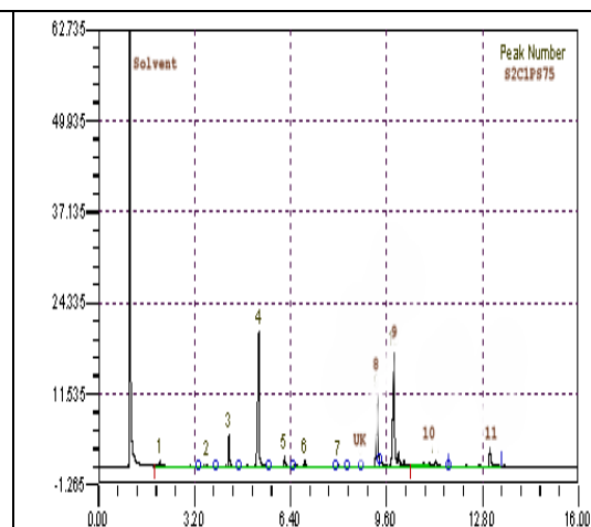
Fig.(4): G. L .C analysis of volatile oil of plant treated with C1 + PS75 2 nd season
