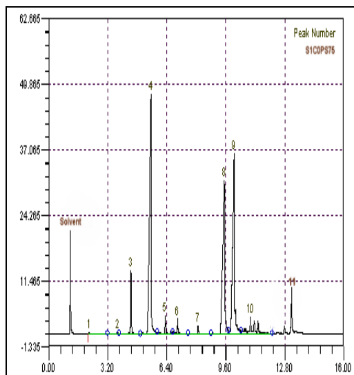
Fig.(1): G. L .C analysis of volatile oil of plant treated with C0 + PS75 1ST season
