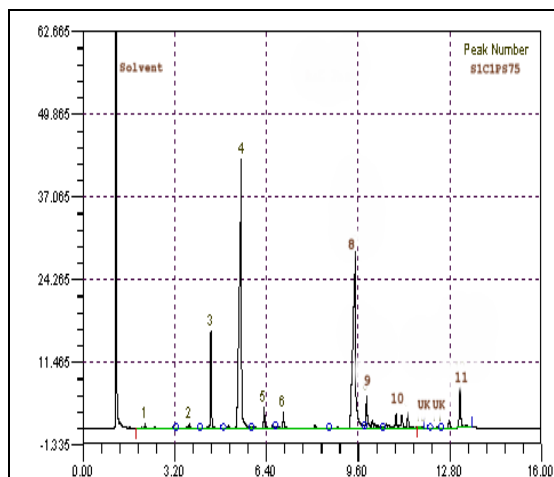
Fig.(3): G. L .C analysis of volatile oil of plant treated with C1 + PS75 1 ST season
