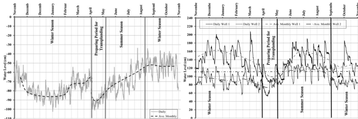
Figure 2. Daily and monthly water levels of wells installed in the study area
